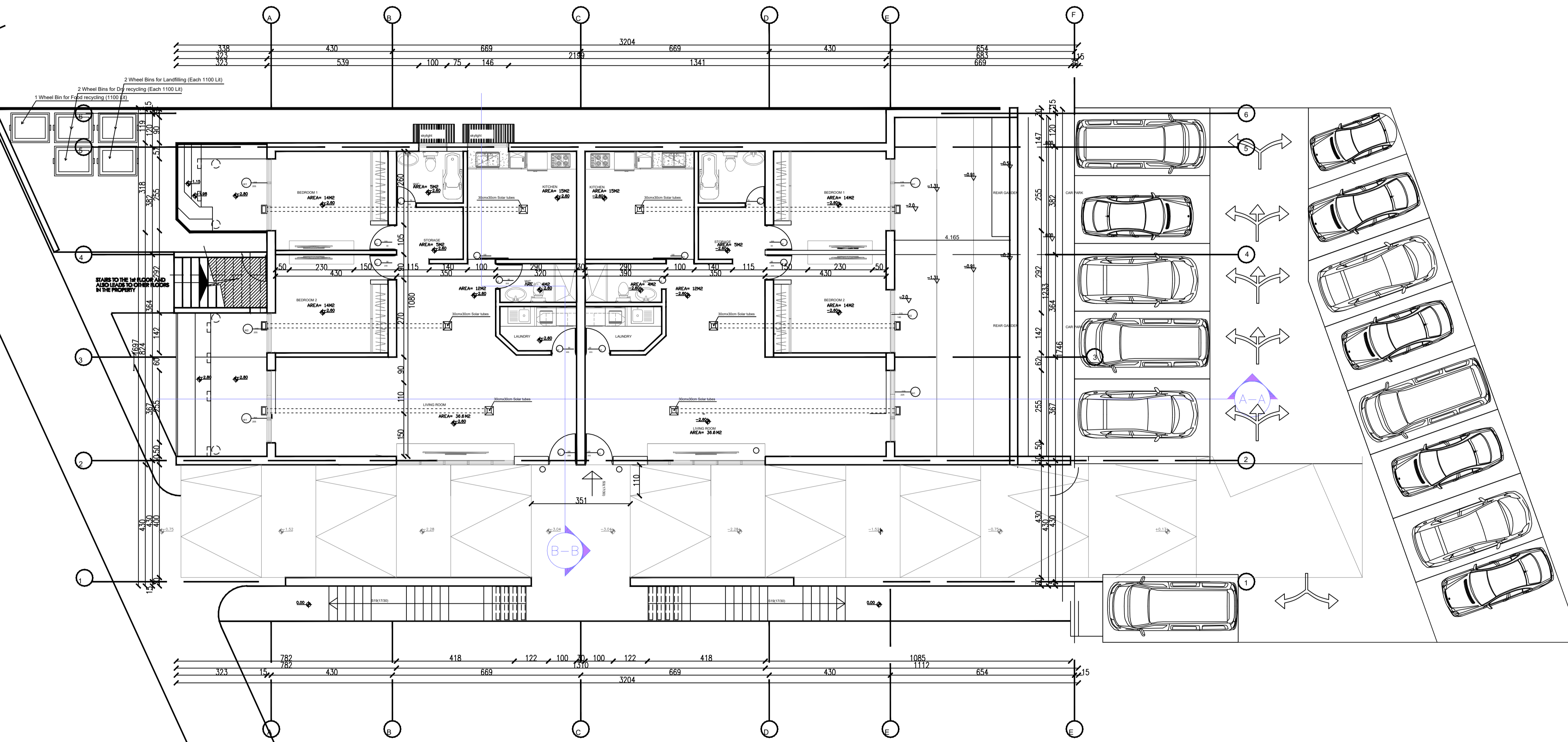
BASEMENT PLAN 1:100
