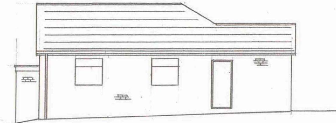
EXISTING SIDE ELEVATION FROM N°7
