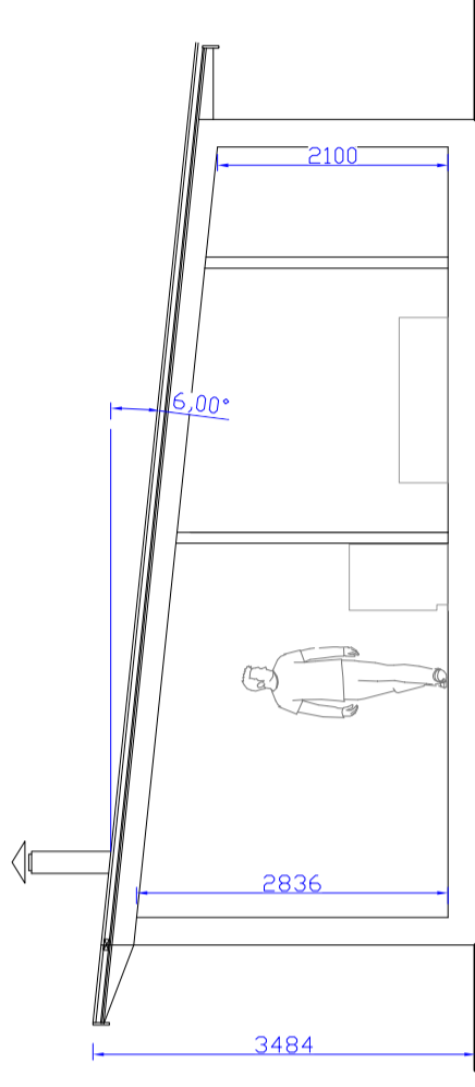
Section
