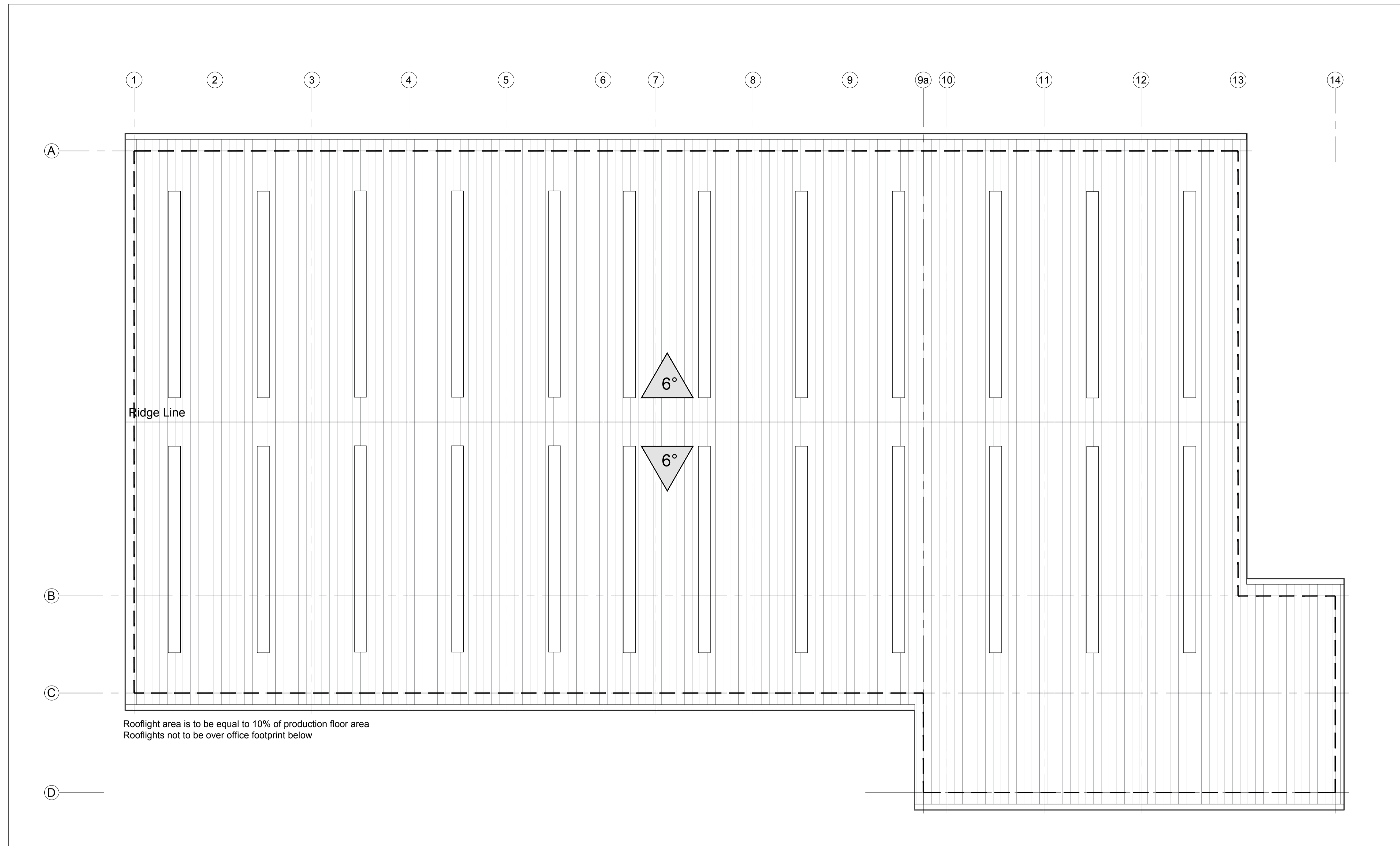
01 Unit 6 Roof Plan 1:200 @ A1
