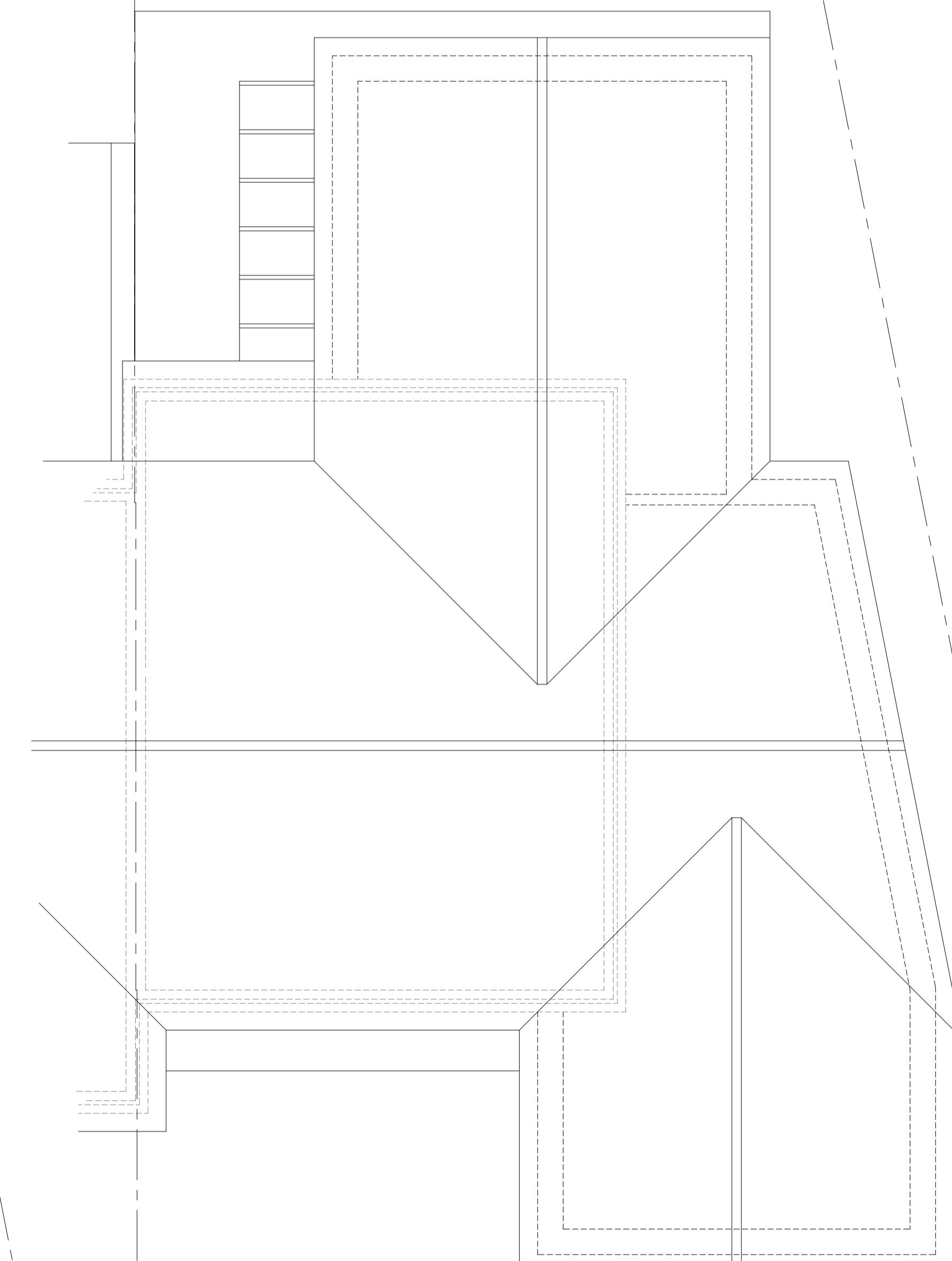
PROPOSED ROOF PLAN Scale 1:50
