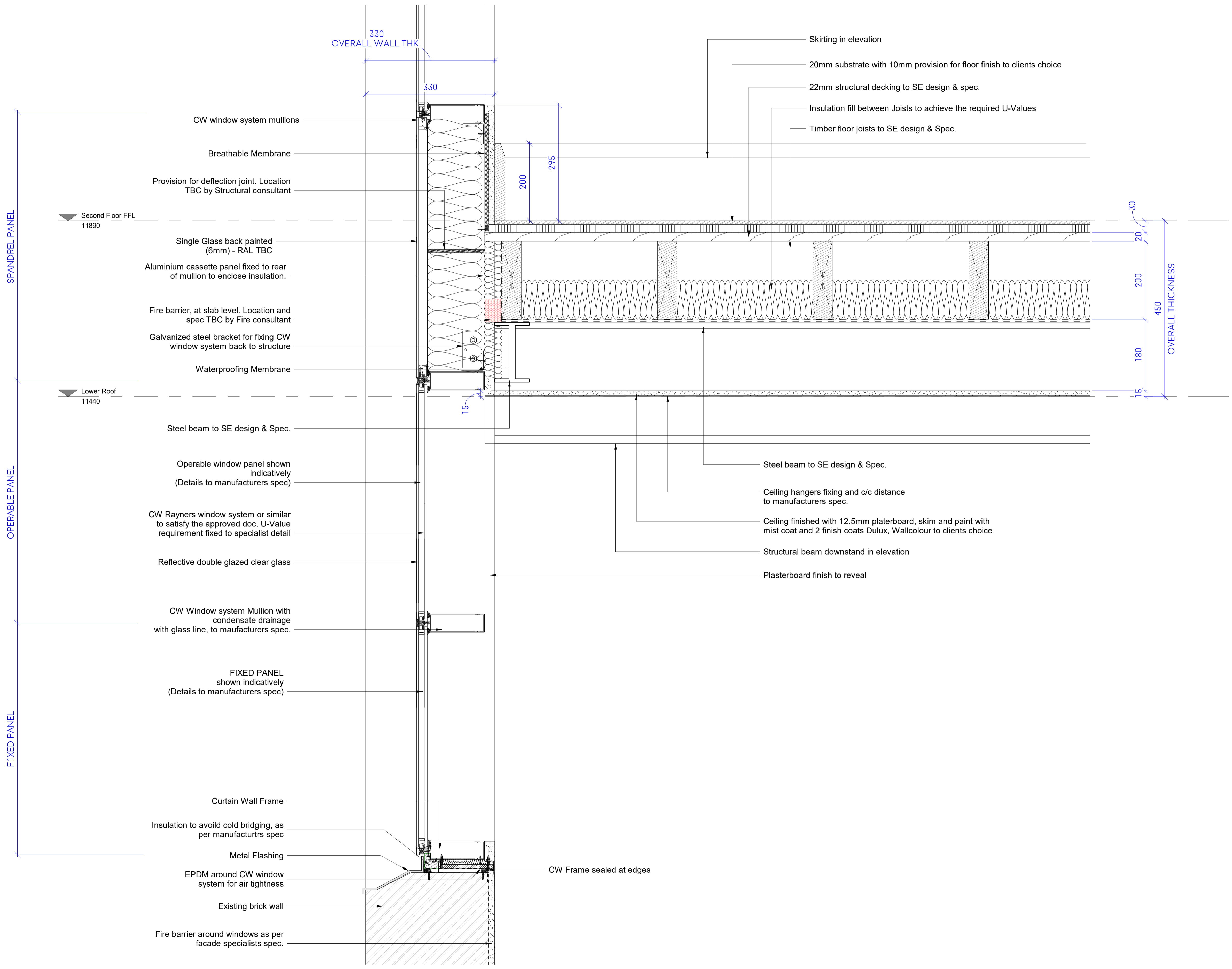
1 Wall to New Floor Junction (Second Floor) 1 : 5
