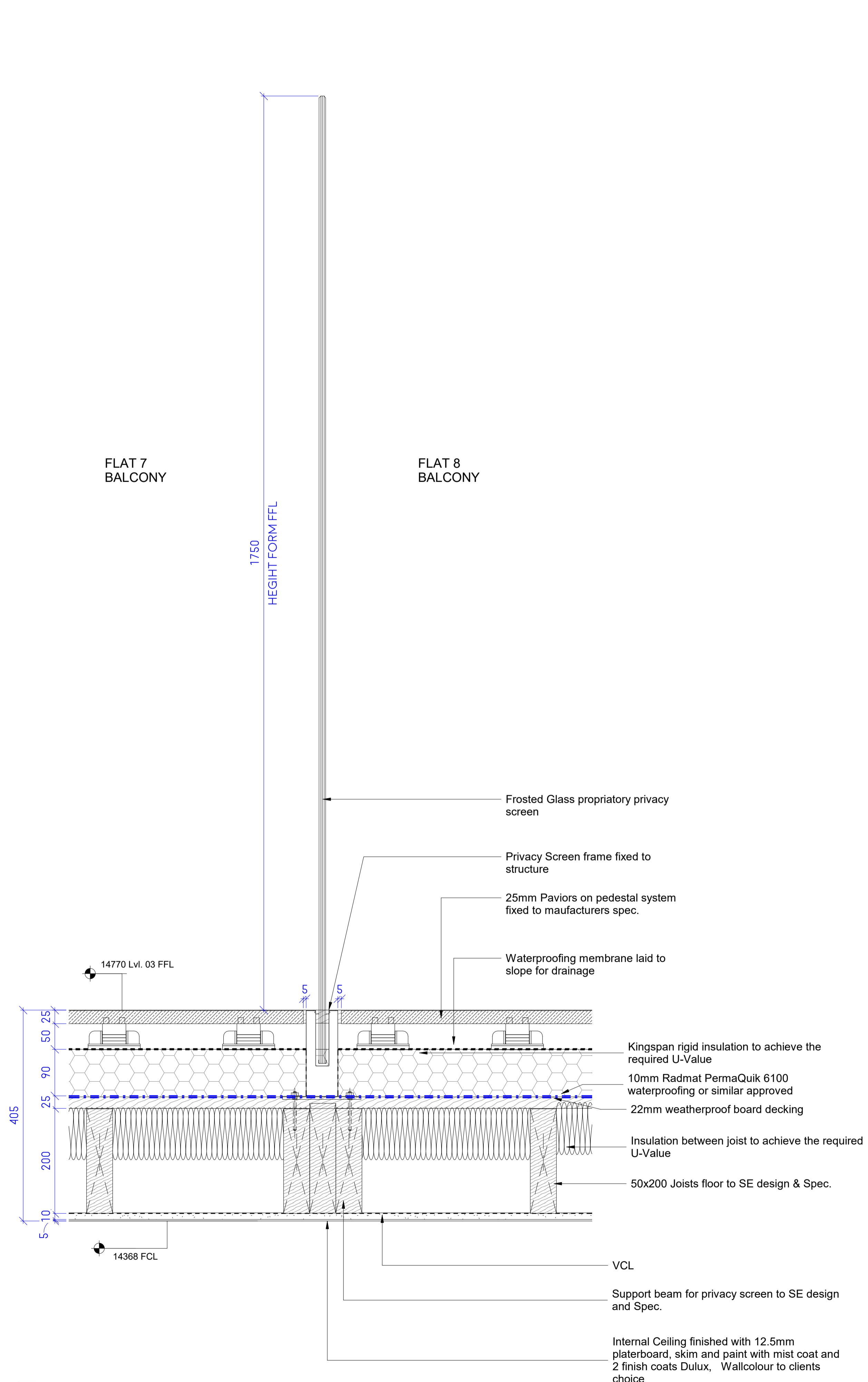
1 Privacy Screen Detail 1 : 5
