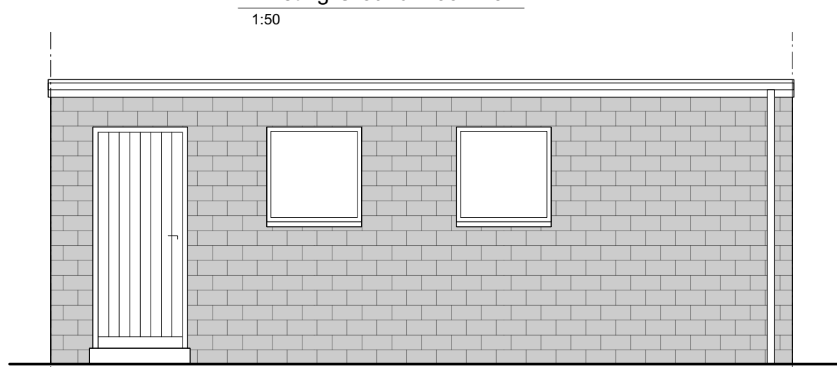
Existing Elevation to Rear Garden 1:50
