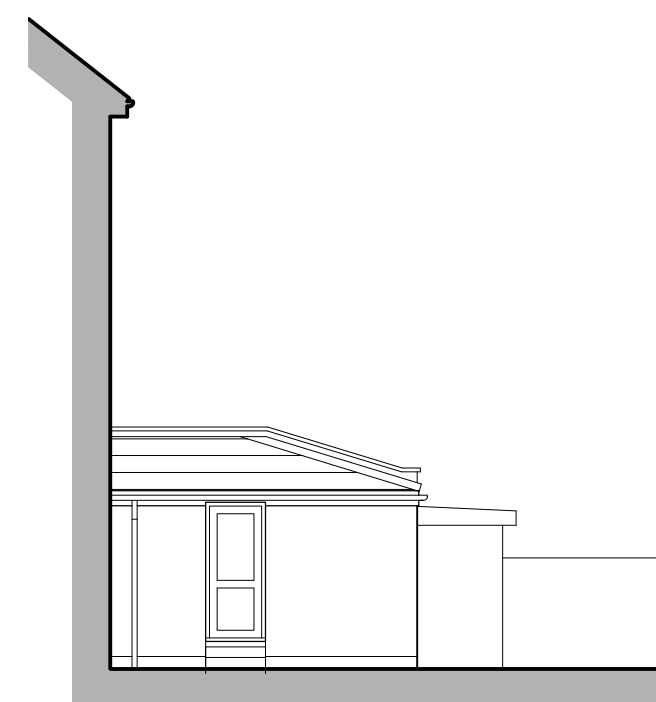
SIDE ELEVATION - EXISTING 1:100
