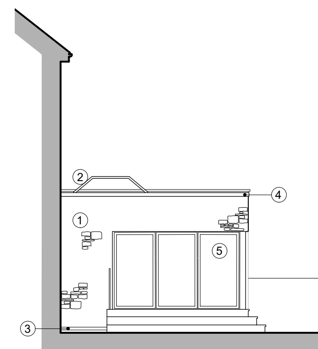
SIDE ELEVATION - PROPOSED 1:100
