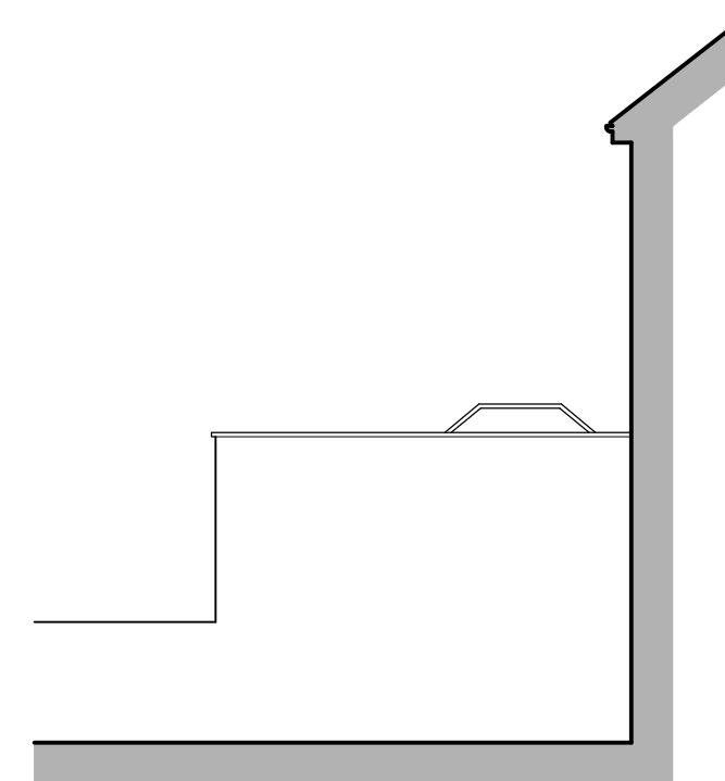
SIDE ELEVATION - (View from no.53) PROPOSED 1:100
