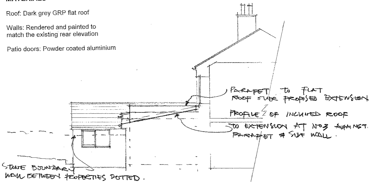
WESTERN ELEVATION FACING NO 3
