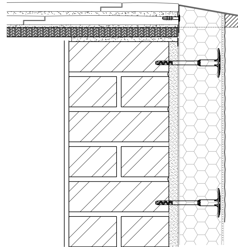
VERGE DETAIL
