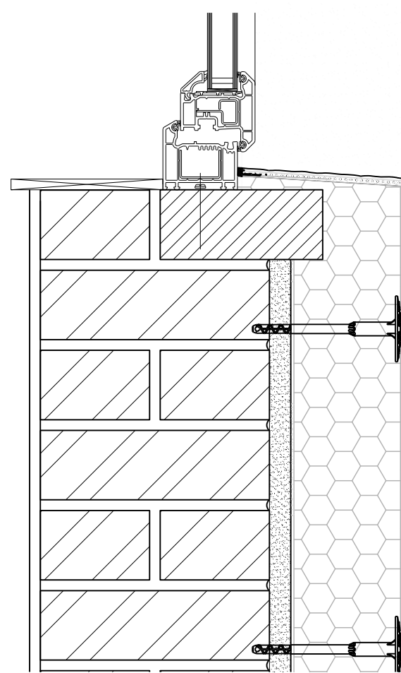
WINDOW CILL DETAIL
