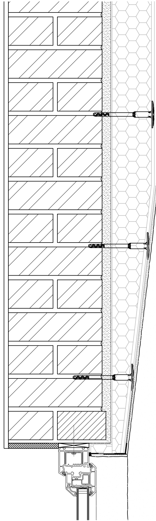
WINDOW DETAIL
