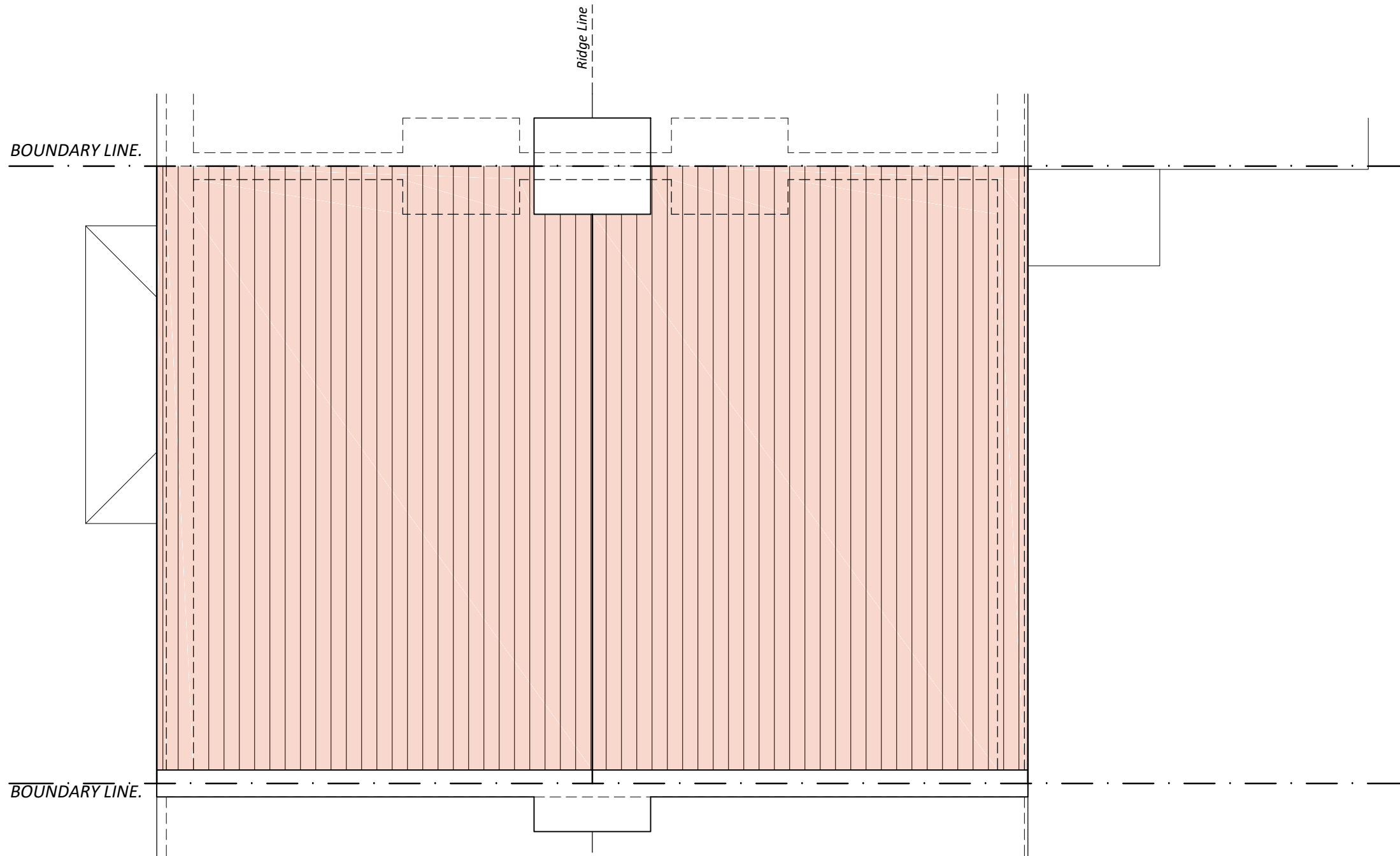
EXISTING ROOF PLAN. SCALE 1:50
