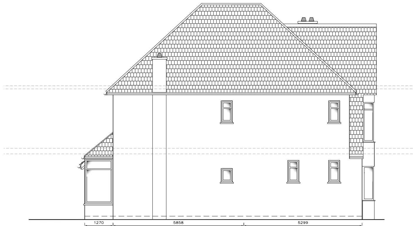
EXISTING SIDE ELEVATION D (1:100)
