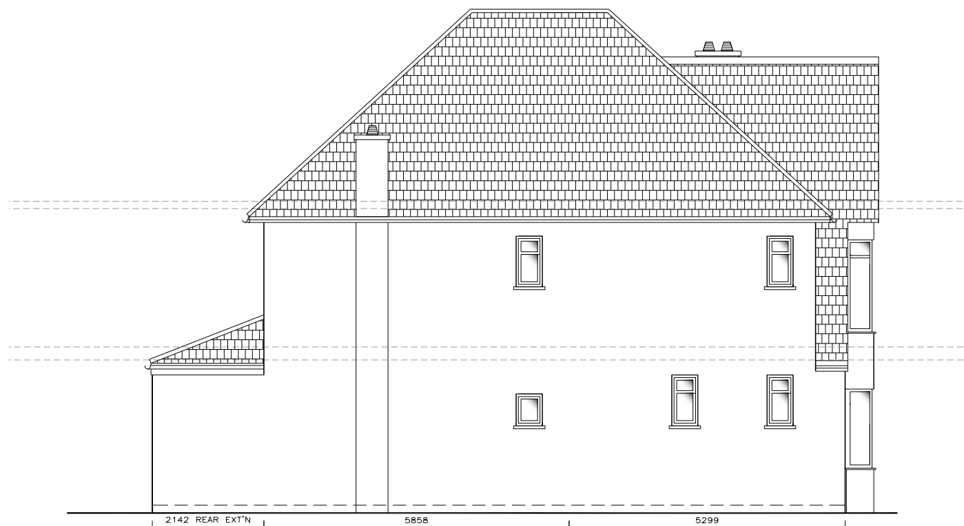
PROPOSED SIDE ELEVATION D (1:100)
