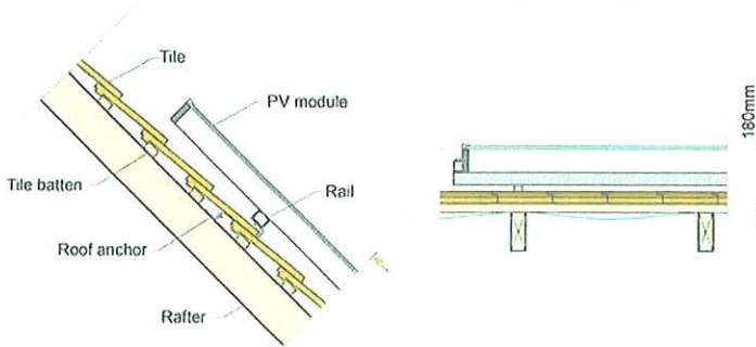
Rack-Mounted Installation
