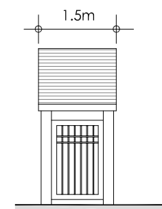
PROPOSED ENTRANCE STRUCTURE SIDE ELEVATION
