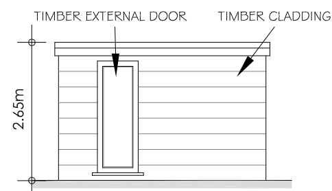
PROPOSED STORE ROOM FRONT ELEVATION
