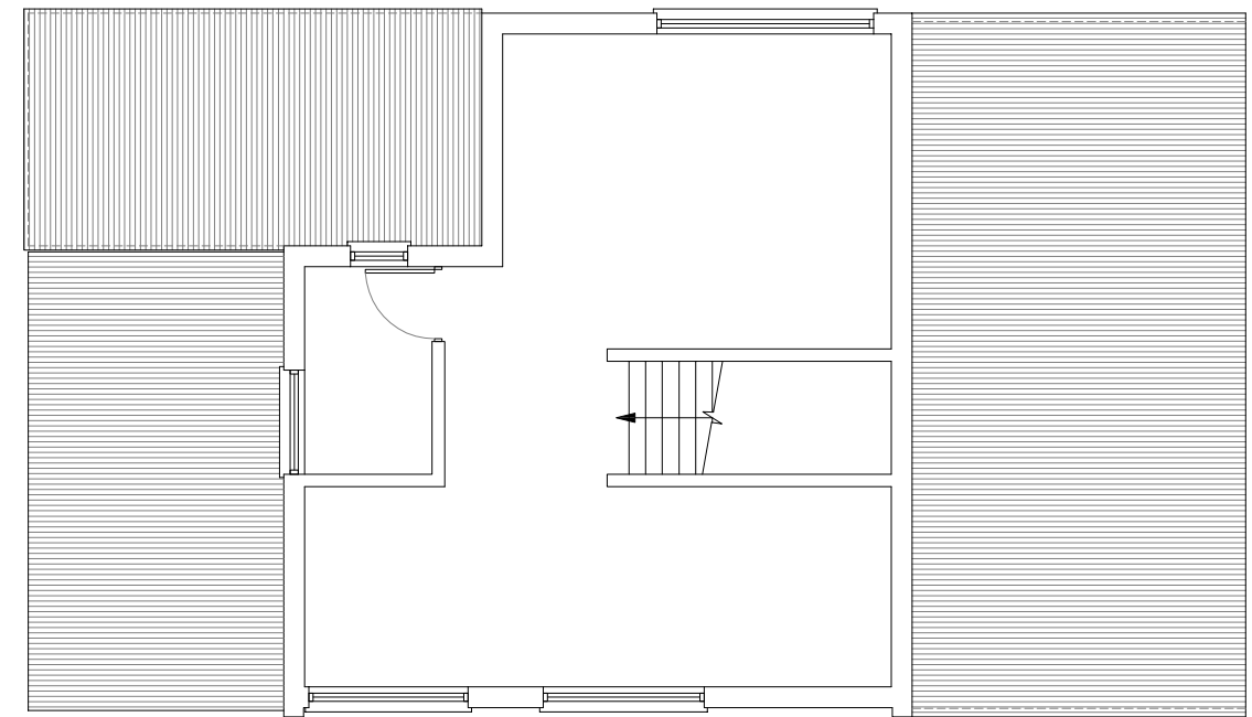
PROPOSED FIRST FLOOR PLANS
