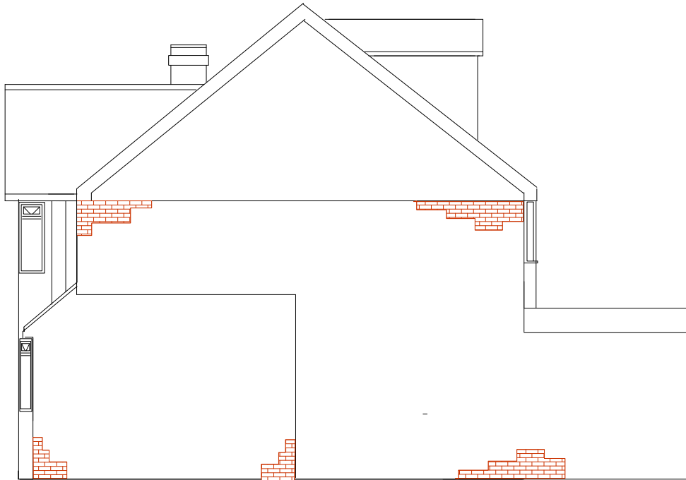
7. Proposed Side (S) Elevation
