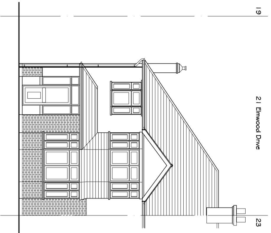
Existing Front Elevation Scale : 1/100@A4
