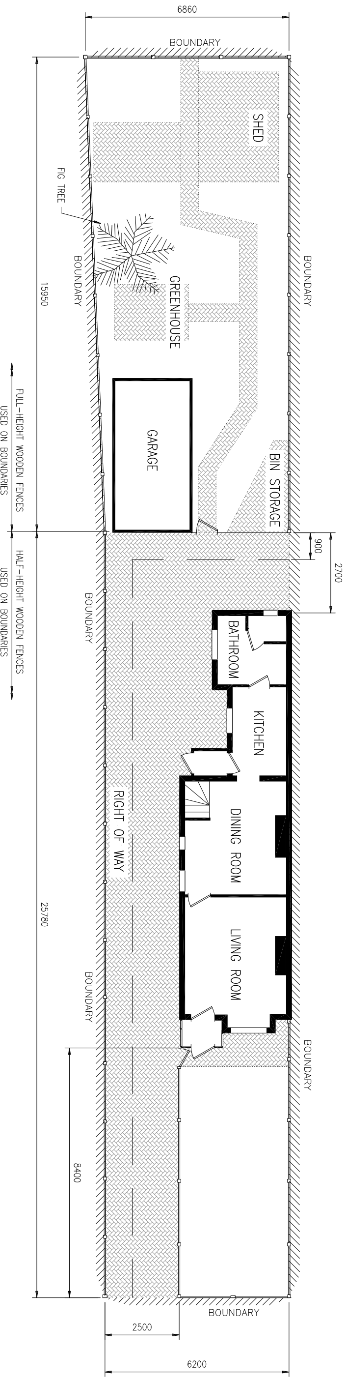
SITE PLAN
