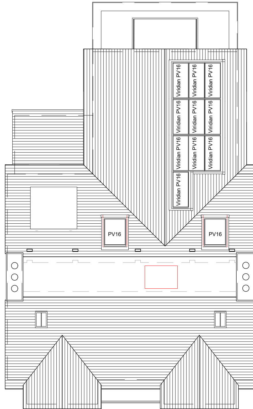
Roof Plan
