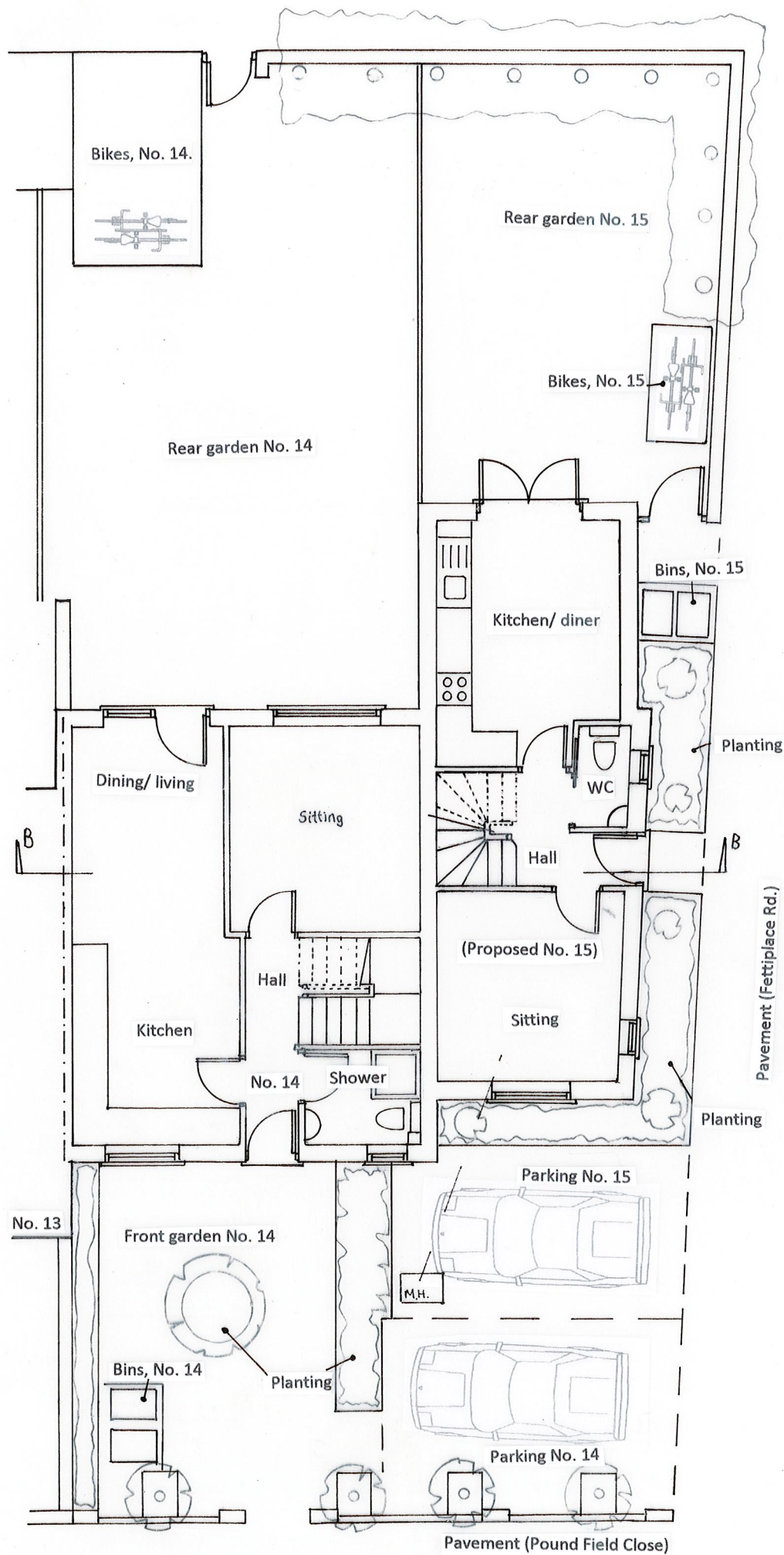
GROUND FLOOR/ SITE/ BLOCK PLAN
