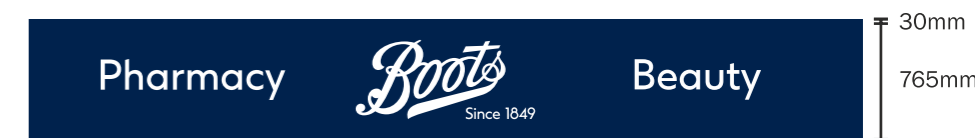
Sign D Cornmarket st fascias Fascia Size: 5,510mm x 765mm + 30mm upstand 3mm aluminium powder coated to match RAL 5013, supplied with fixing rails, 100mm deep. 'Boots since 1849' cut in 10mm 1T77 LED acrylic, pushed through approx 5mm, Acrylic category text cut in 8mm opal 050 acrylic, pushed through approx 3mm, all acrylic being back lit with LED trays. Cap height of 'P' in Pharmacy = 203mm Logo height: 520mm
