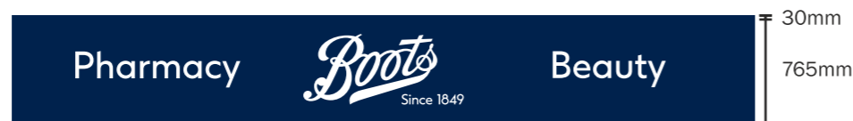
Sign B Cornmarket st fascias Fascia Size: 5,490mm x 765mm + 30mm upstand 3mm aluminium powder coated to match RAL 5013, supplied with fixing rails, 100mm deep. 'Boots since 1849' cut in 10mm 1T77 LED acrylic, pushed through approx 5mm. Acrylic category text cut in 8mm opal 050 acrylic, pushed through approx 3mm, all acrylic being back lit with LED trays. Cap height of 'P' in Pharmacy = 203mm Logo height: 520mm
