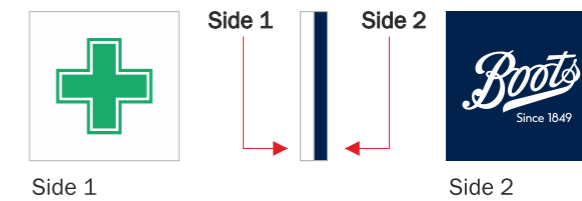
Sign G 600 x 600mm projecting sign - fit to Centre of Right Fascia graphic cut in projecting sign, backed and pushed through opal acrylic, green vinyl to face of cross, approx 2 / 3mm projecting*, back illuminated with LED, lighting tray to rear of cross. Logo height: 520mm
