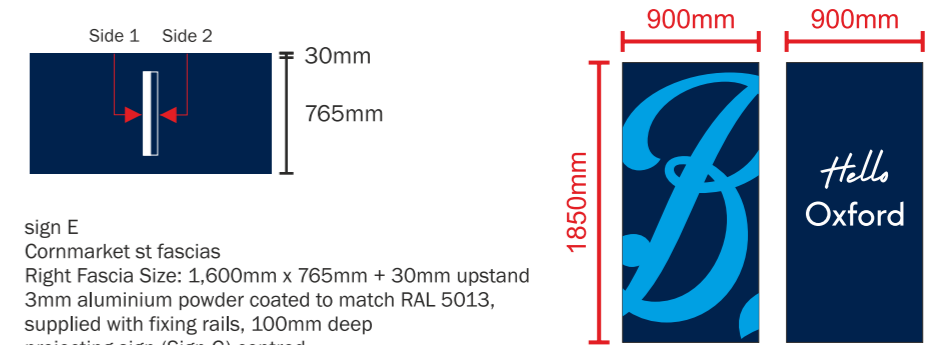
Sign F Welcome tray panels Sizes as Shown 3mm aluminium powder coated to match RAL 5013, supplied with fixing rails,
