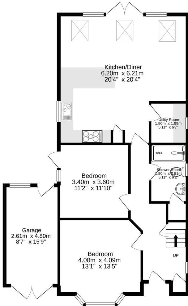
Ground floor 95.7 sq.m. (1030 sq.ft.) approx.
