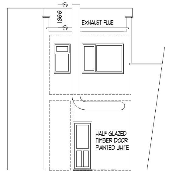
PROPOSED REAR ELEVATION 2
