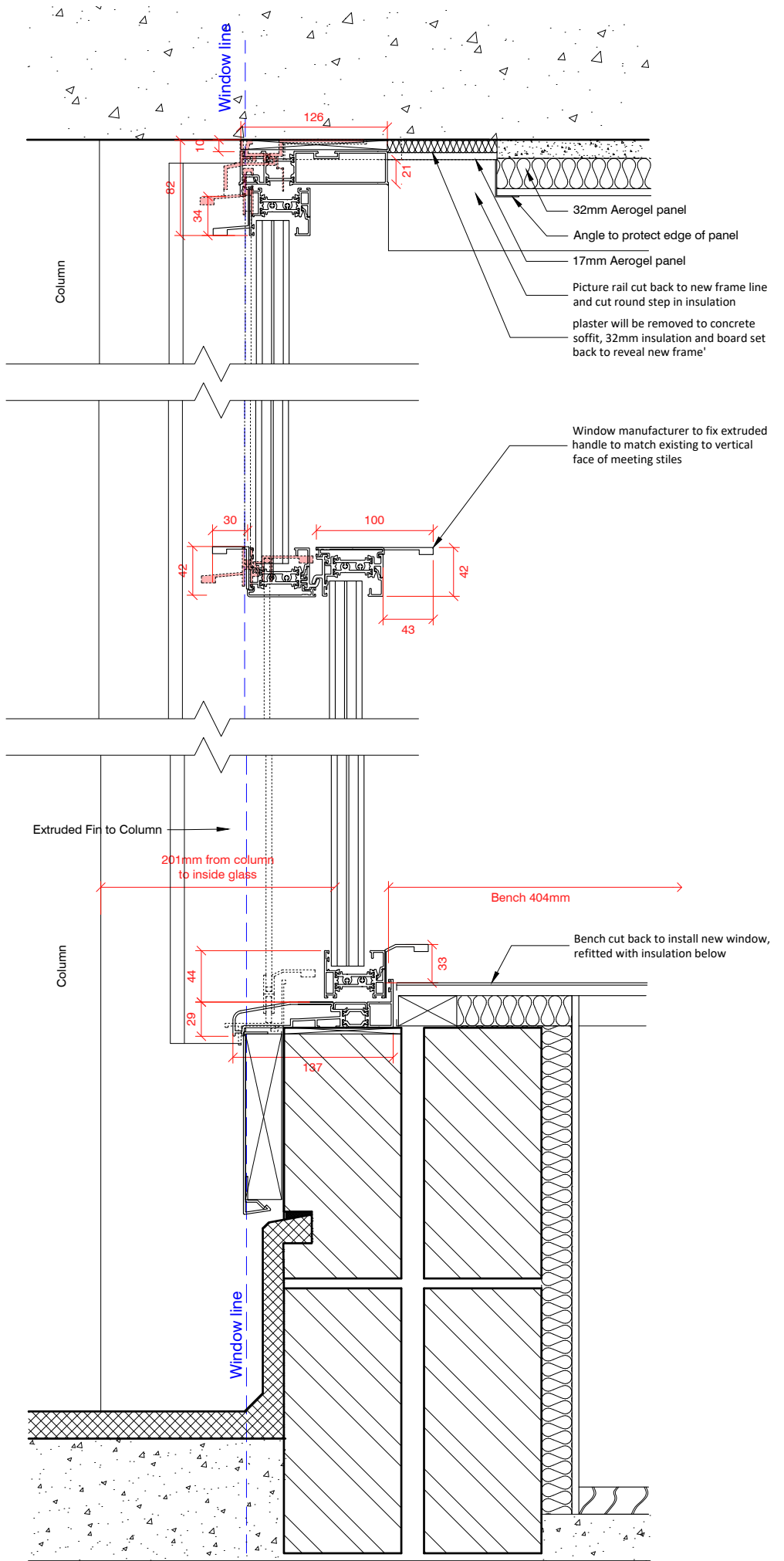
2 Proposed Section Details of Type 2 at Student rooms of Block B, C 1:5
