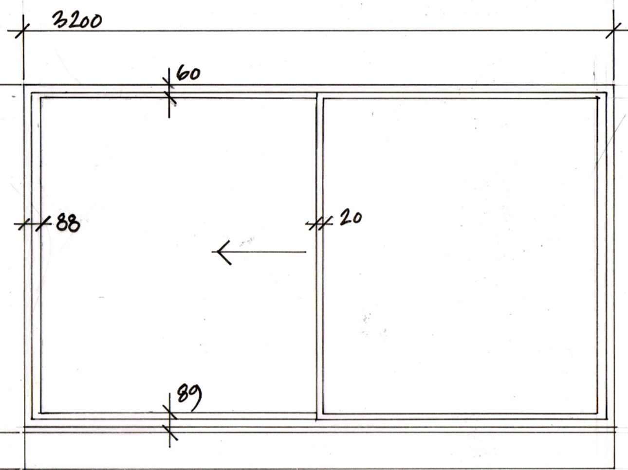
TYPE 1a PROPOSED ELEVATION HORIZONTAL SLIDING.
