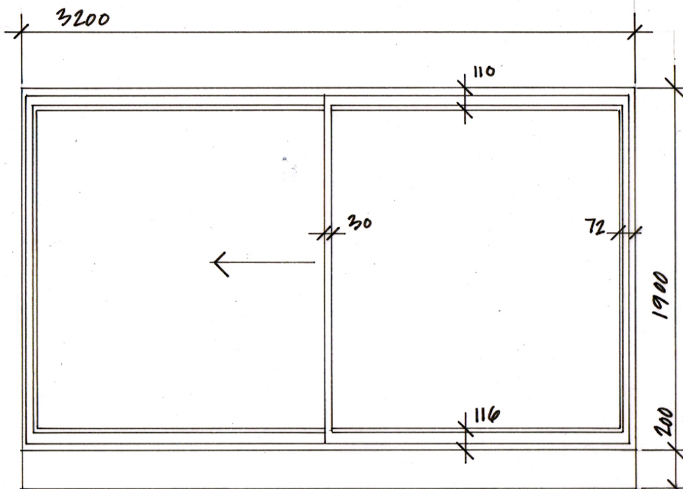
TYPE 1a EXISTING ELEVATION. HORIZONTAL SLIDING
