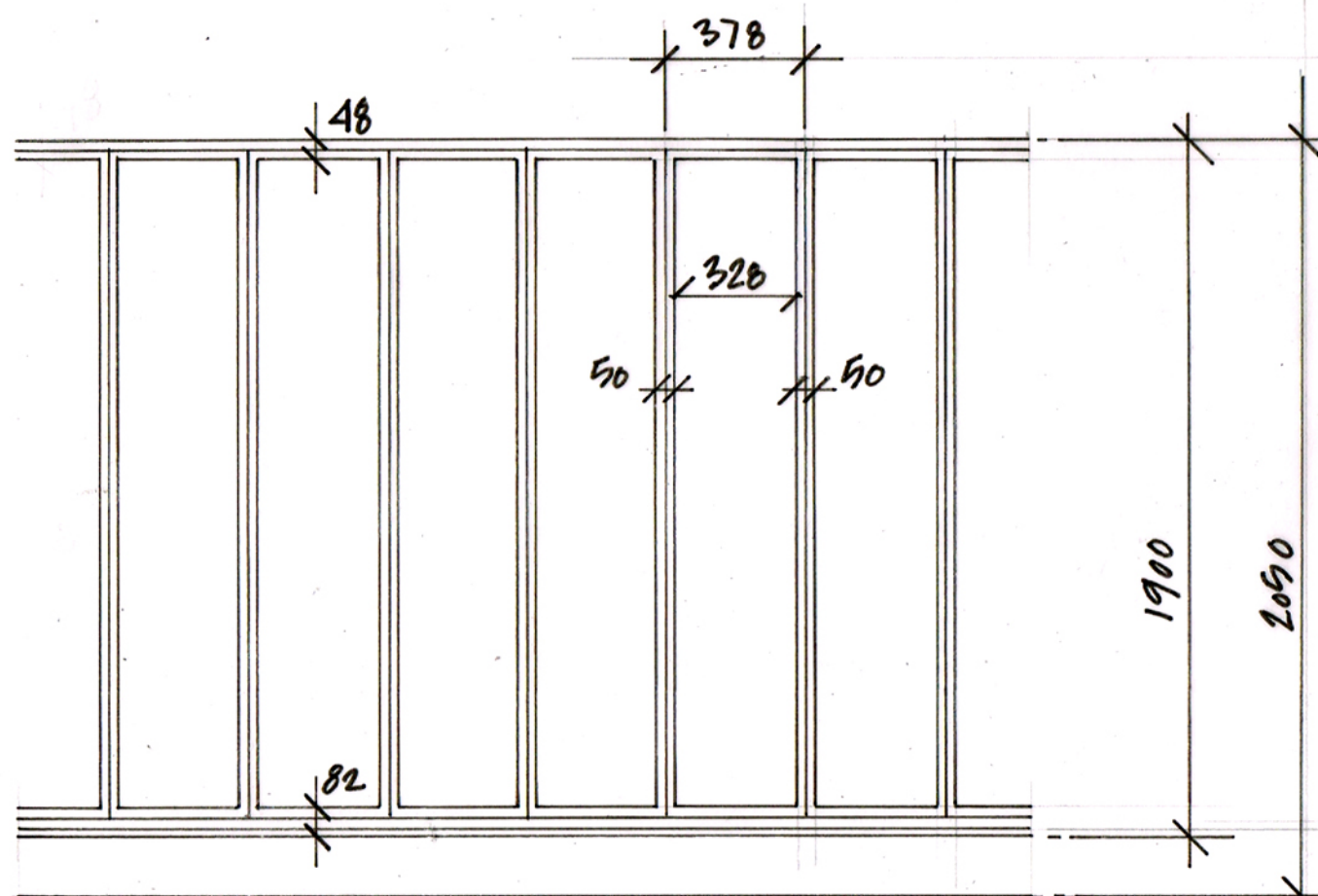
TYPE 9 EXISTING ELEVATION FIXED LIGHTS
