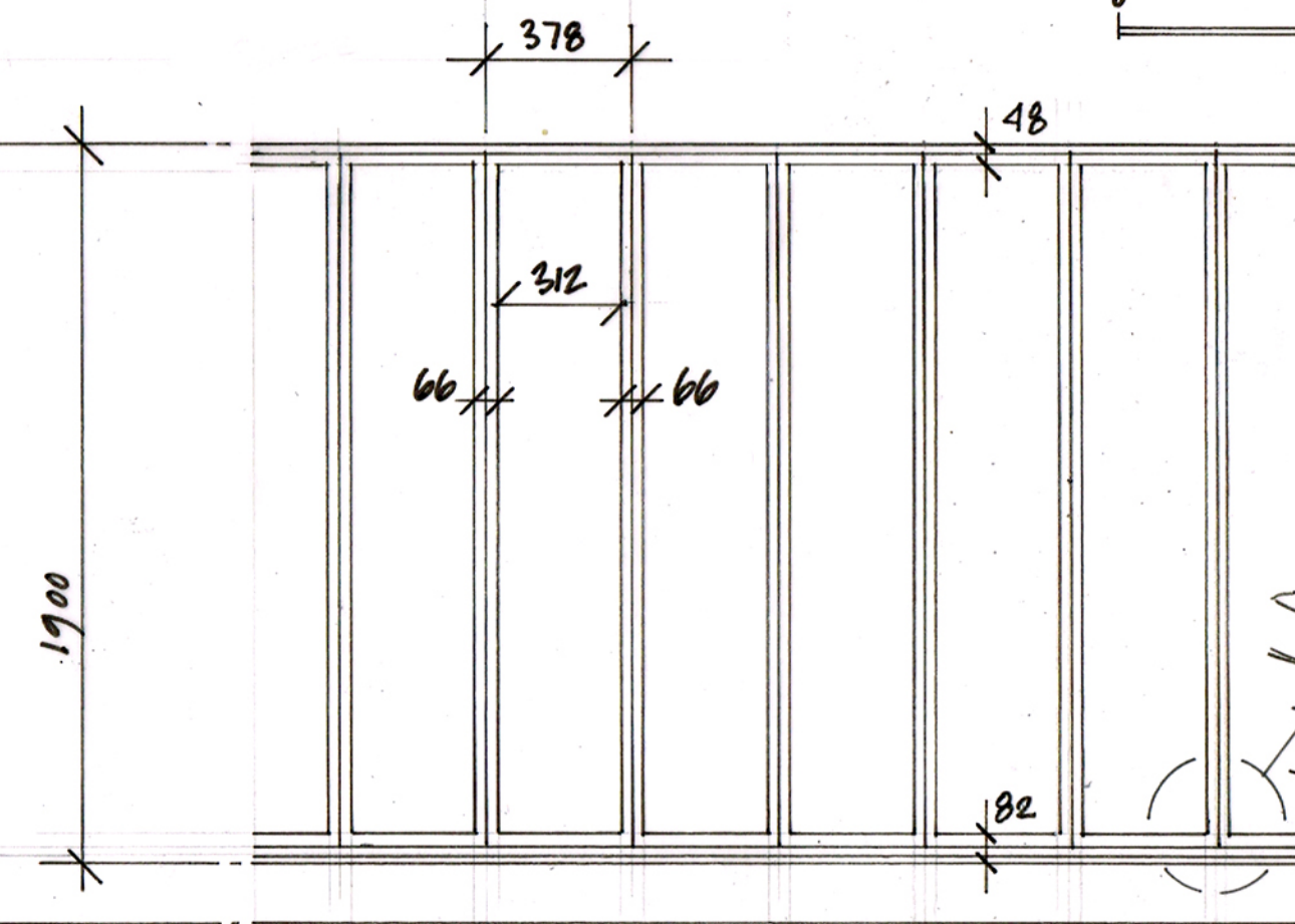
TYPE 9 PROPOSED ELEVATION FIXED LIGHTS.
