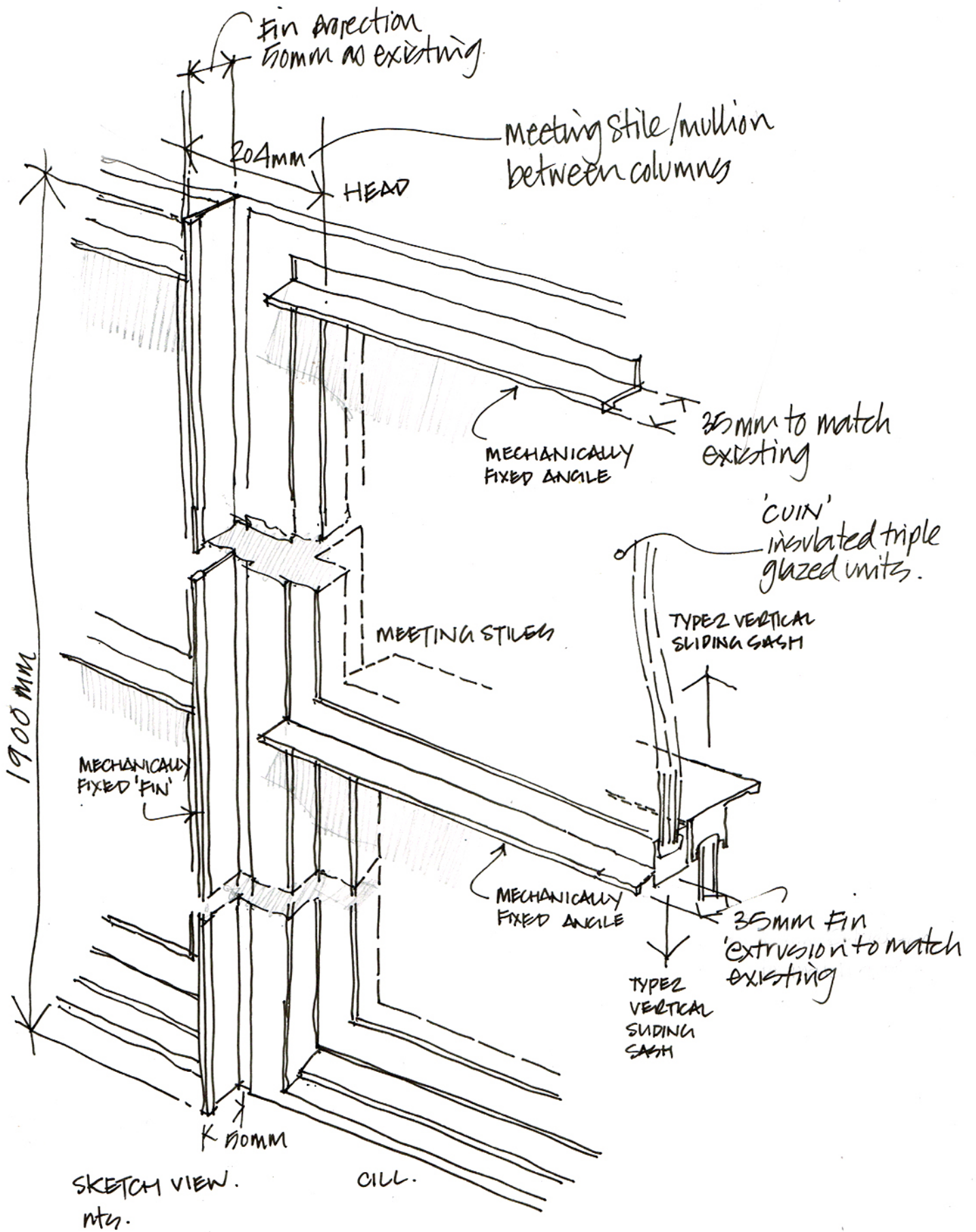
TYPE 2d see drwg PA-73,74 window details + sight line comparison drawing for type 2 - appendix 04.
