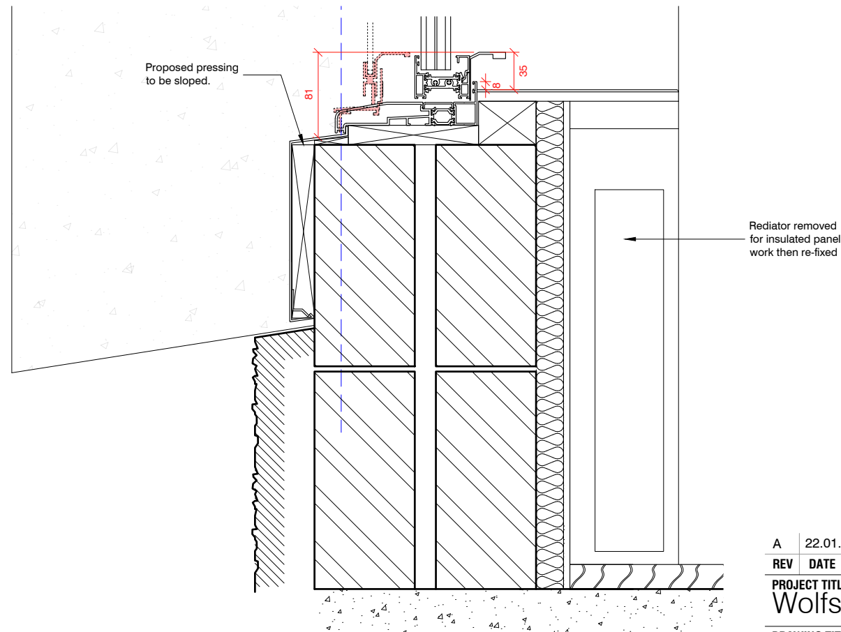
2 Proposed Type 2 Section - Carrells and Library Offices 1:5
