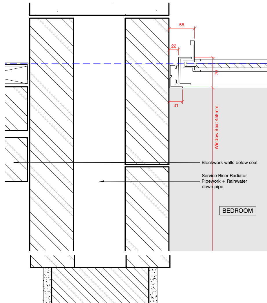
1 Existing Jamb + Below Bench Seat to Type 1 1:5
