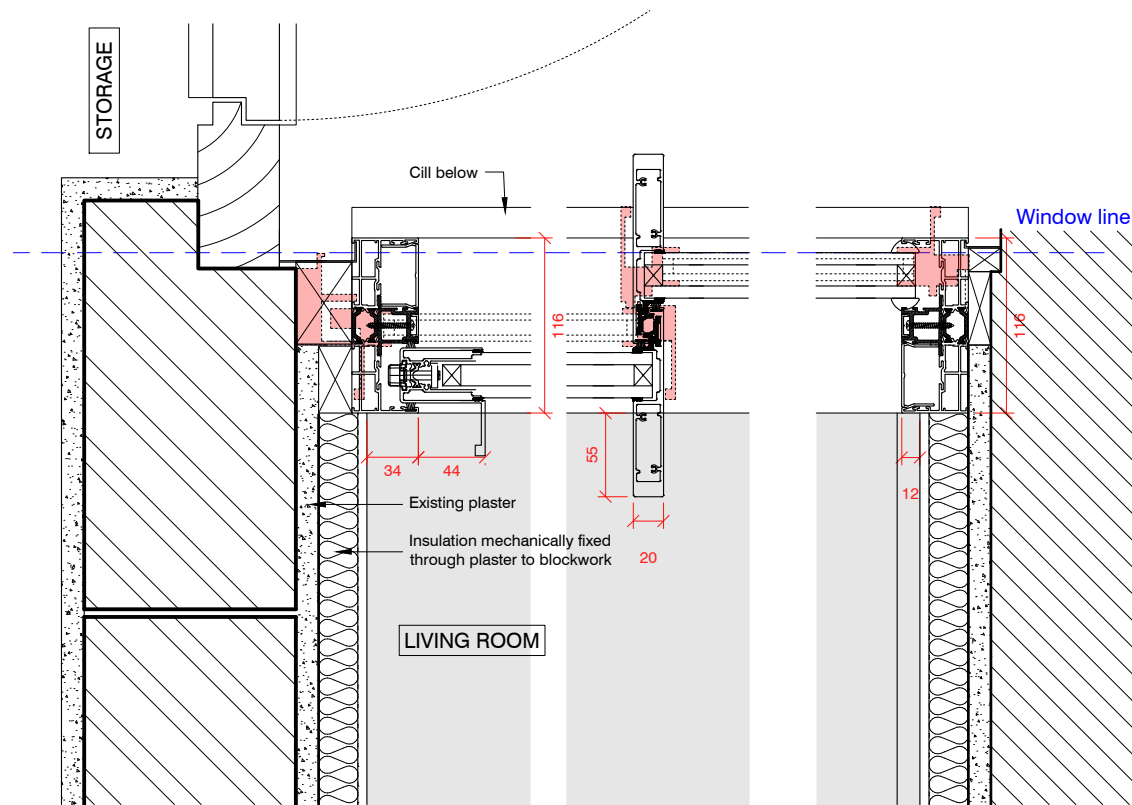
4 Proposed Jamb For Type 1a at Living room of Block F, G, H 1:5
