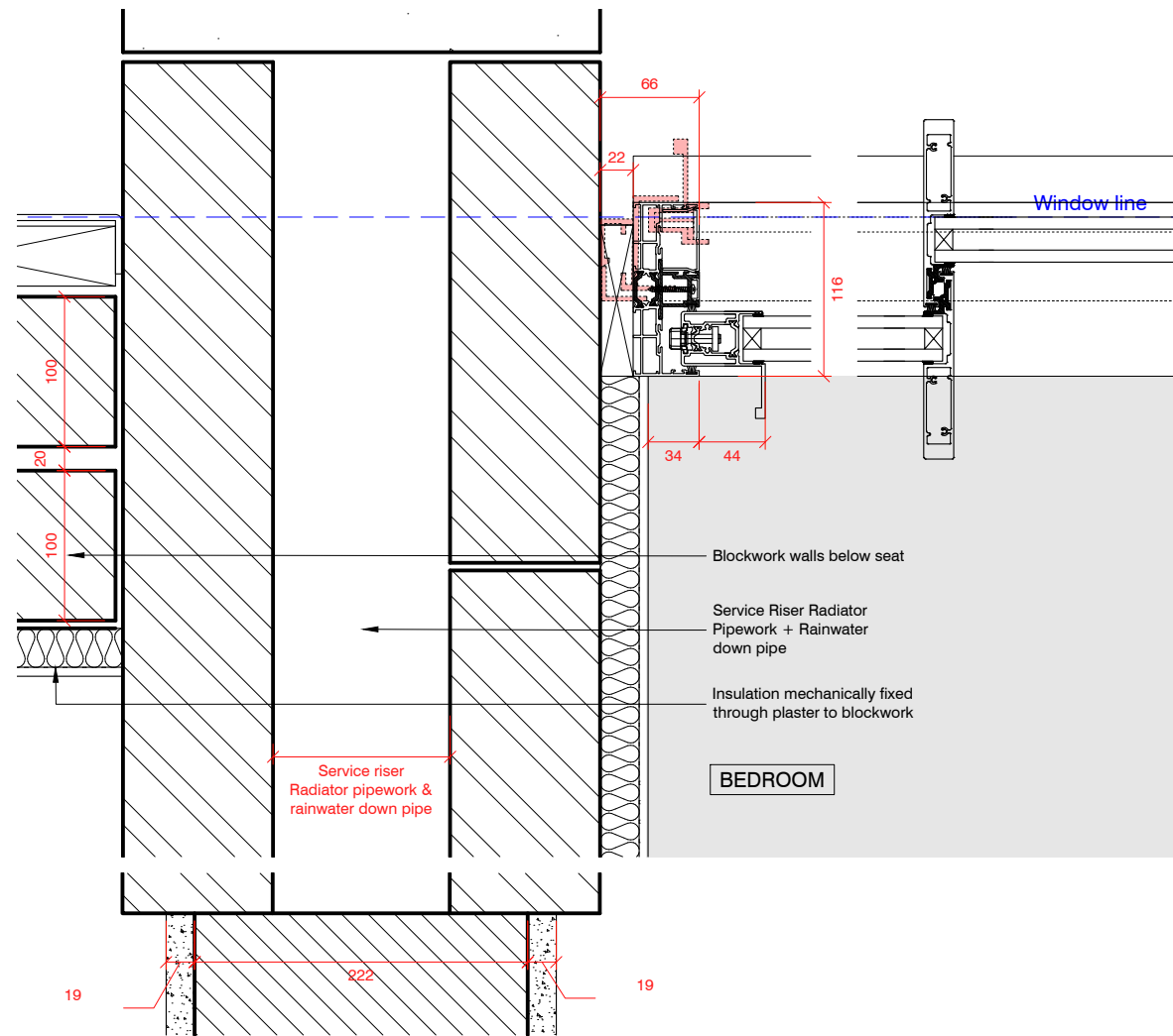
2 Proposed Jamb + Below Bench Seat to Type 1 at Student rooms of Block B, C 1:5
