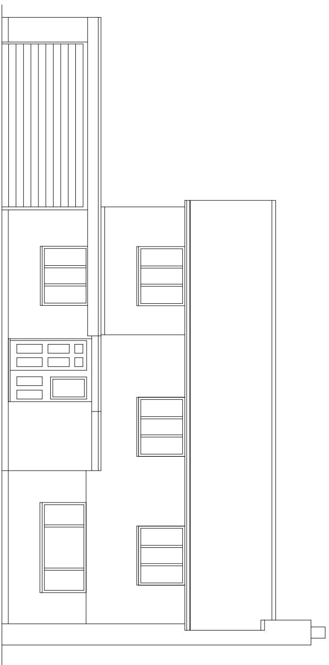
FRONT ELEVATION (EAST)
