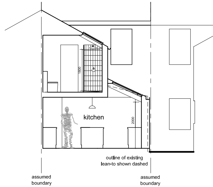
section 1-1
