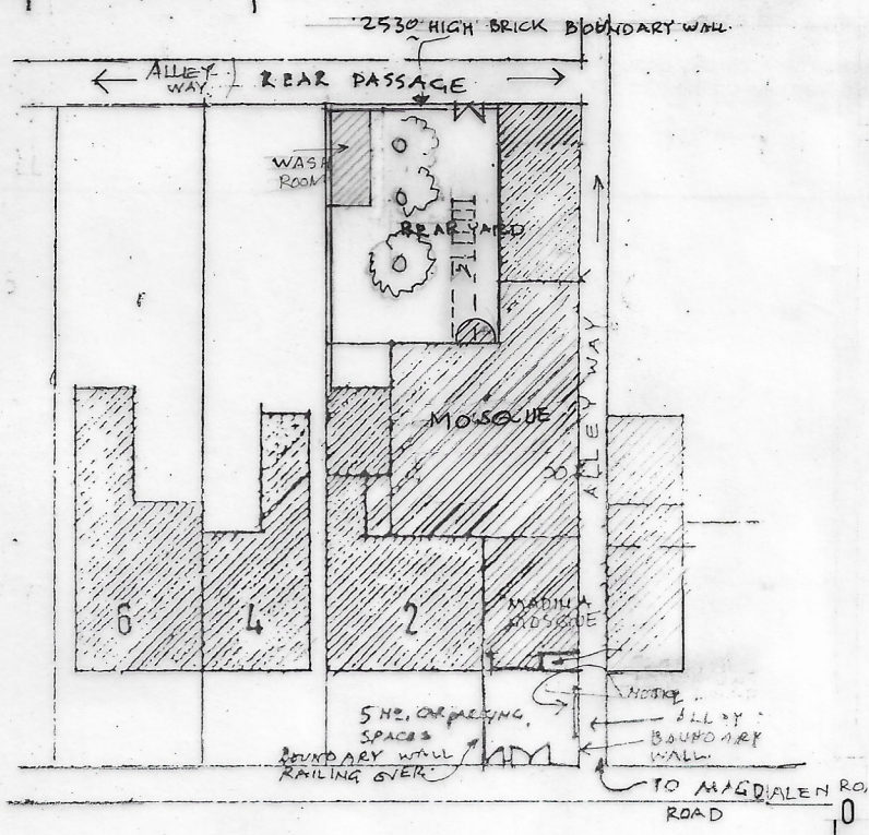
STANLEY ROAD BLOCK PLAN SCALE 1:500
