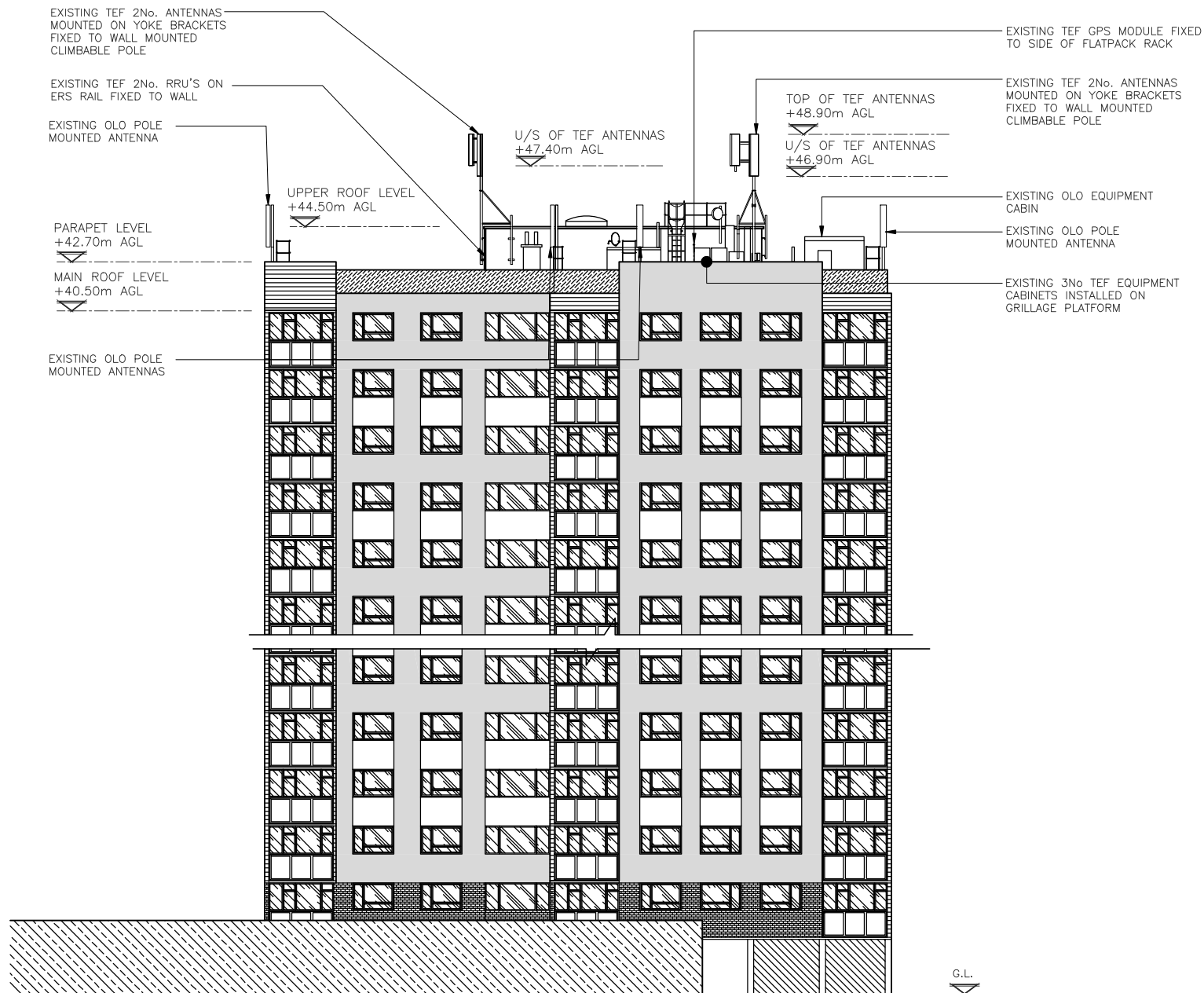
EXISTING WEST ELEVATION (1:200)
