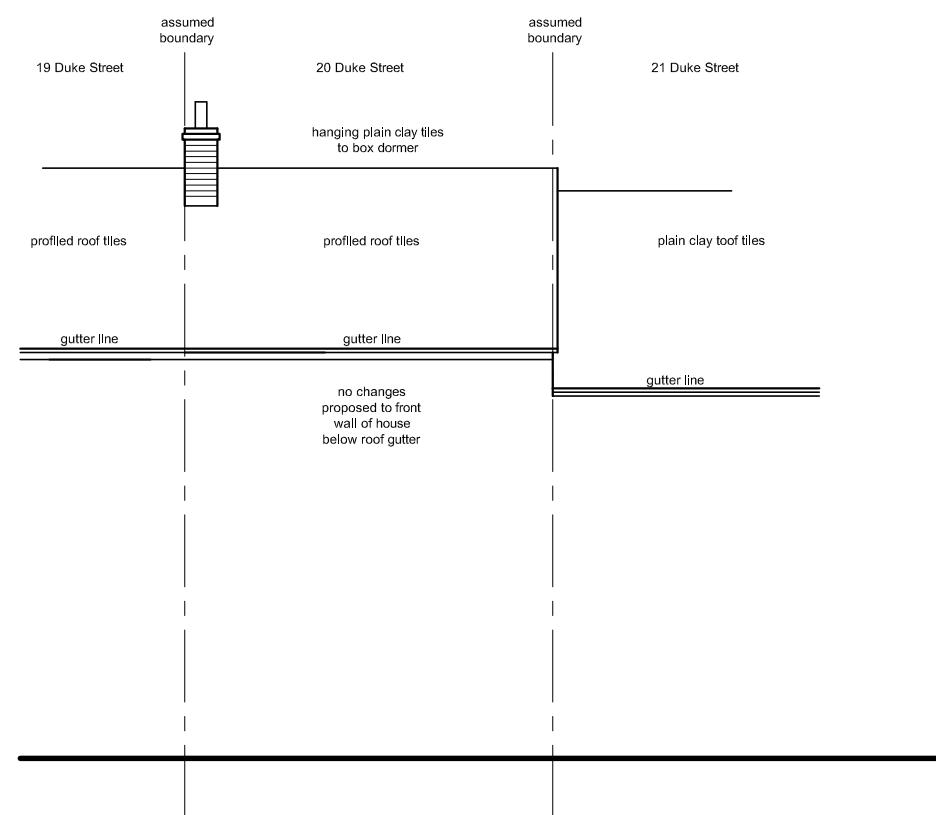
west (front) elevation
