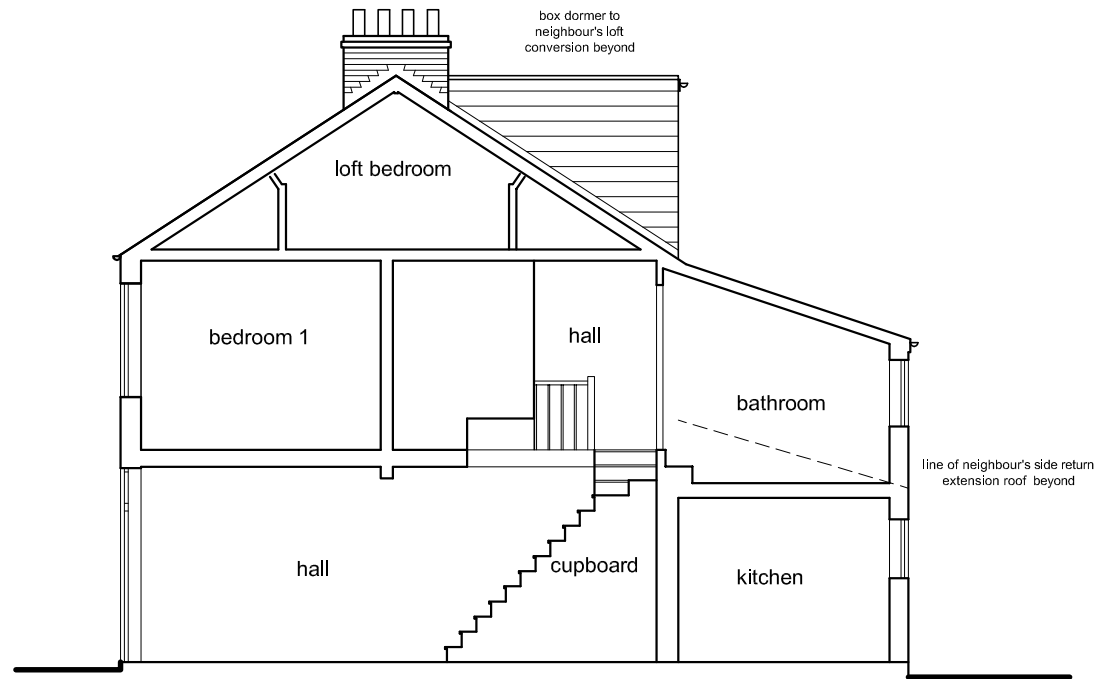
section looking north
