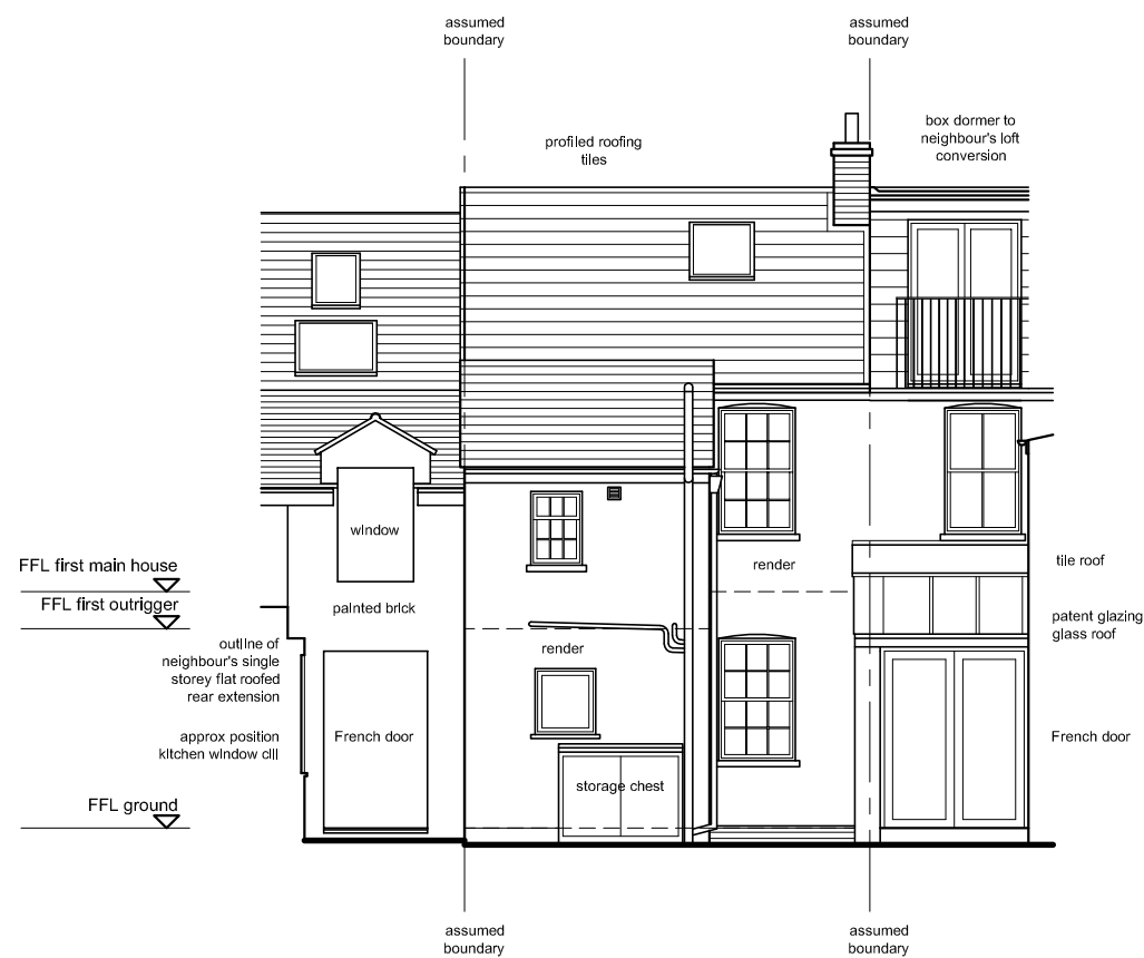
east (rear) elevation
