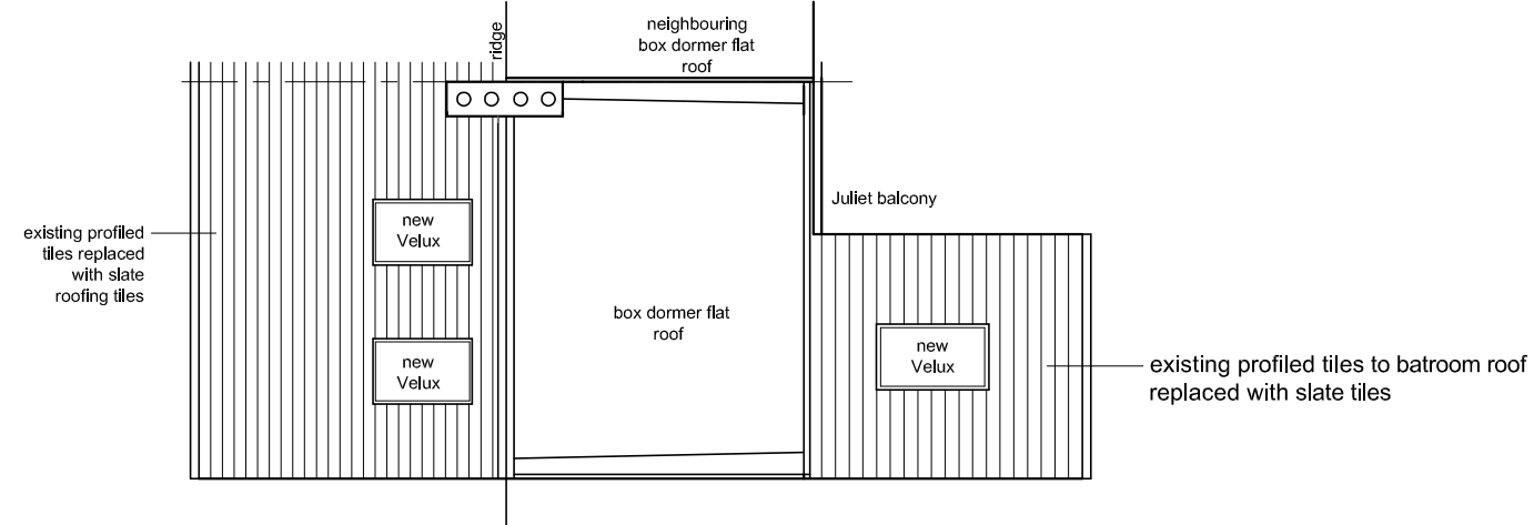
roof plan
