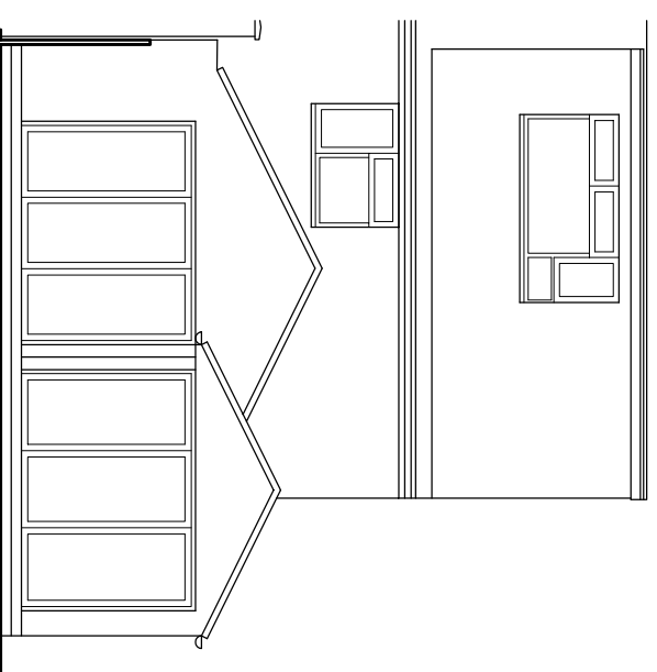
EAST ELEVATION
