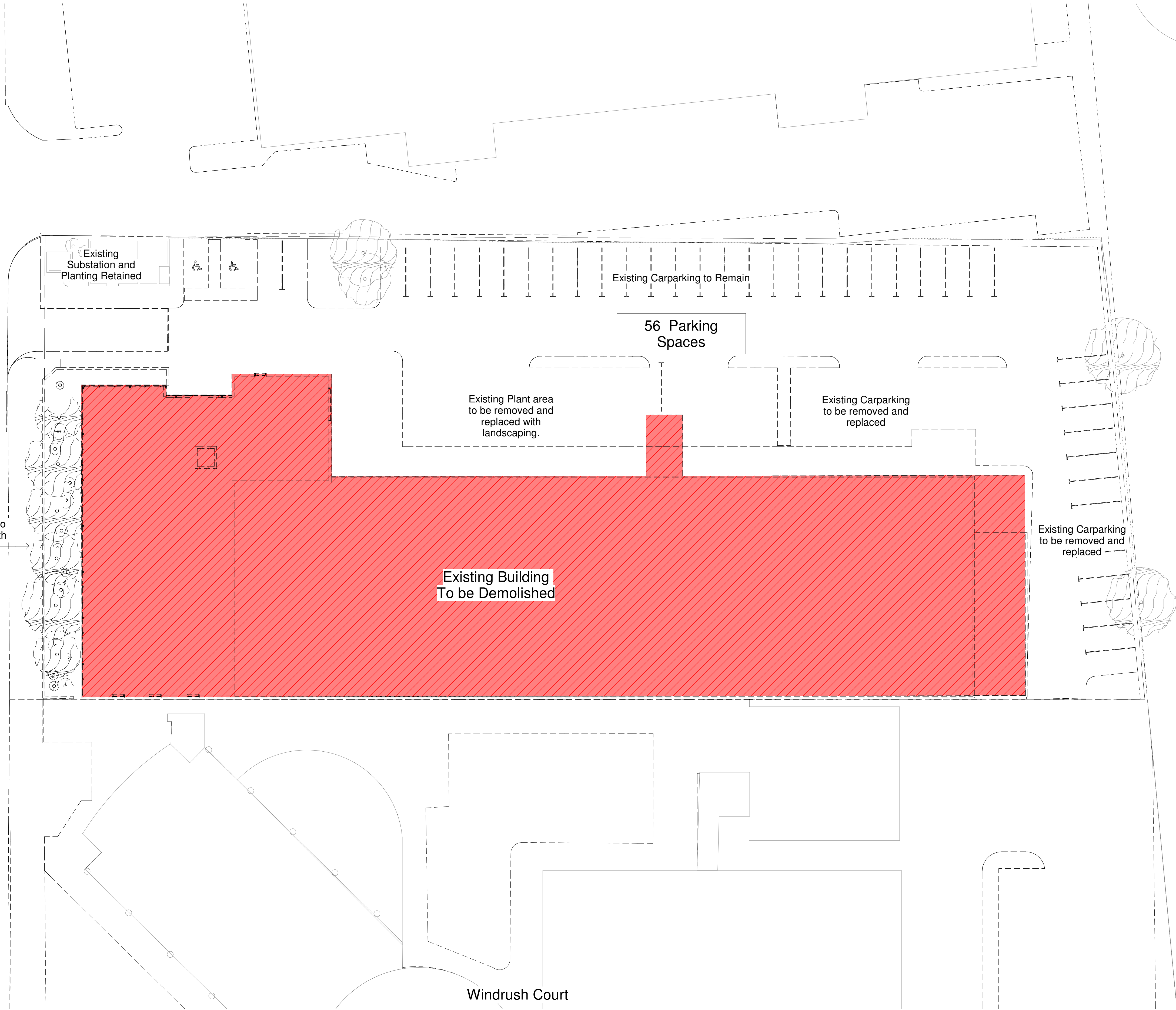
1 Proposed Demolition Plan 1 : 200
