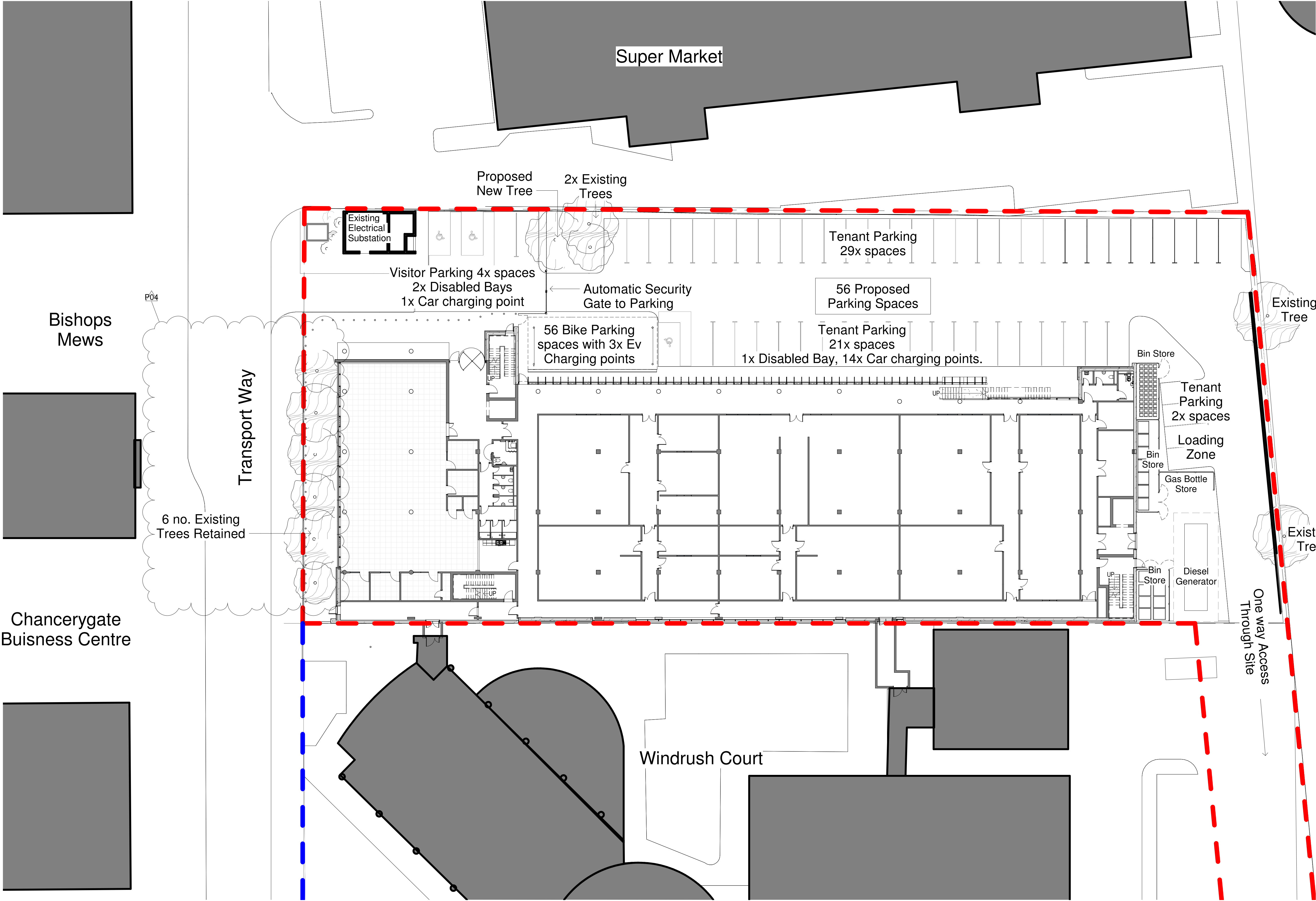
Proposed Site Plan 1 : 200
