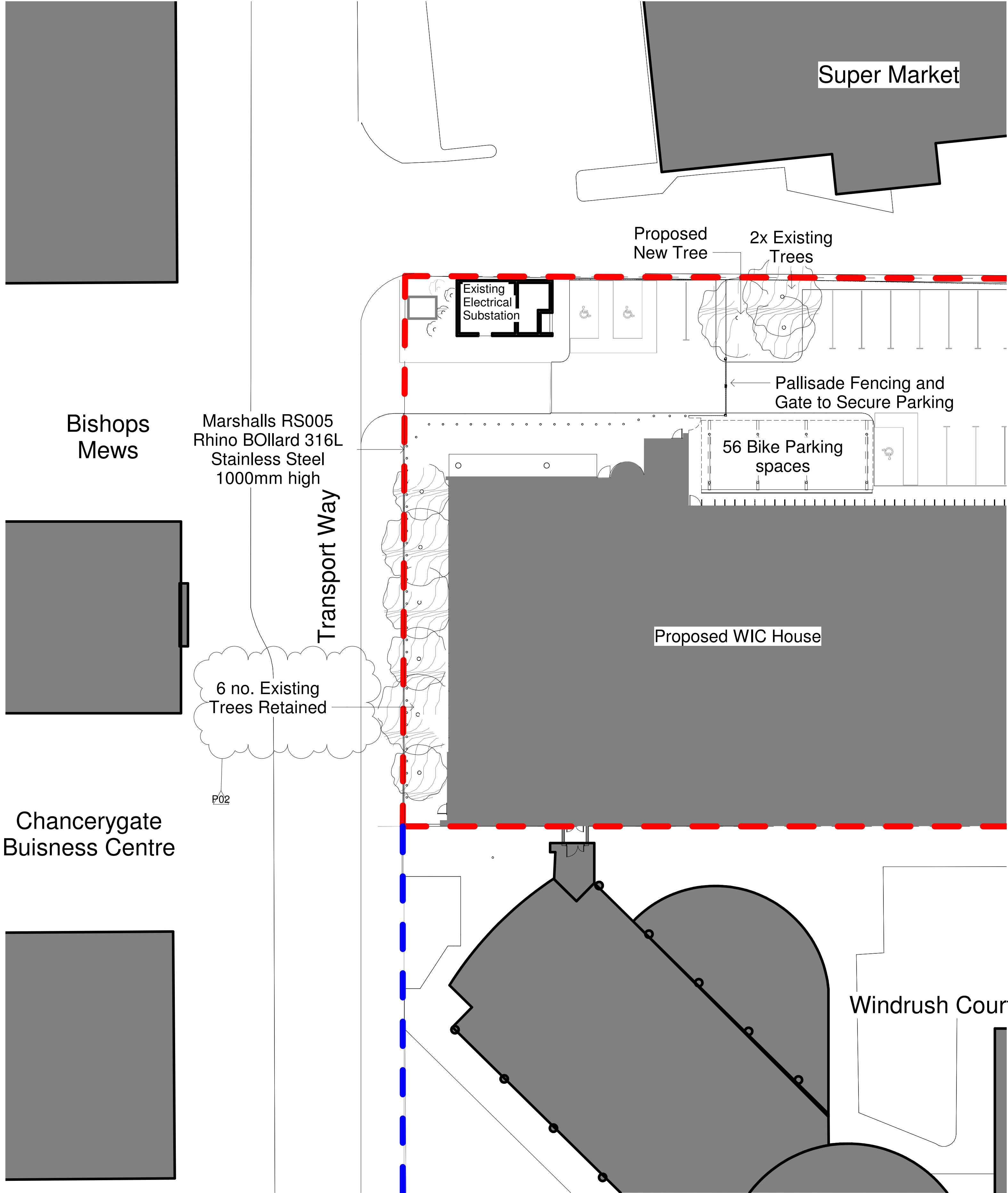
1 Proposed Landscape Plan 1 : 200
