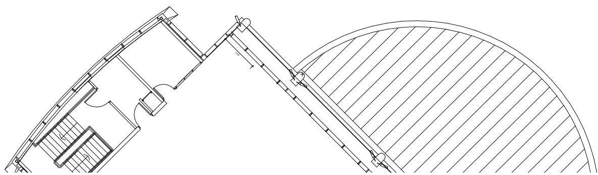
1 Existing Isis House Second Floor Plan 1 : 200
