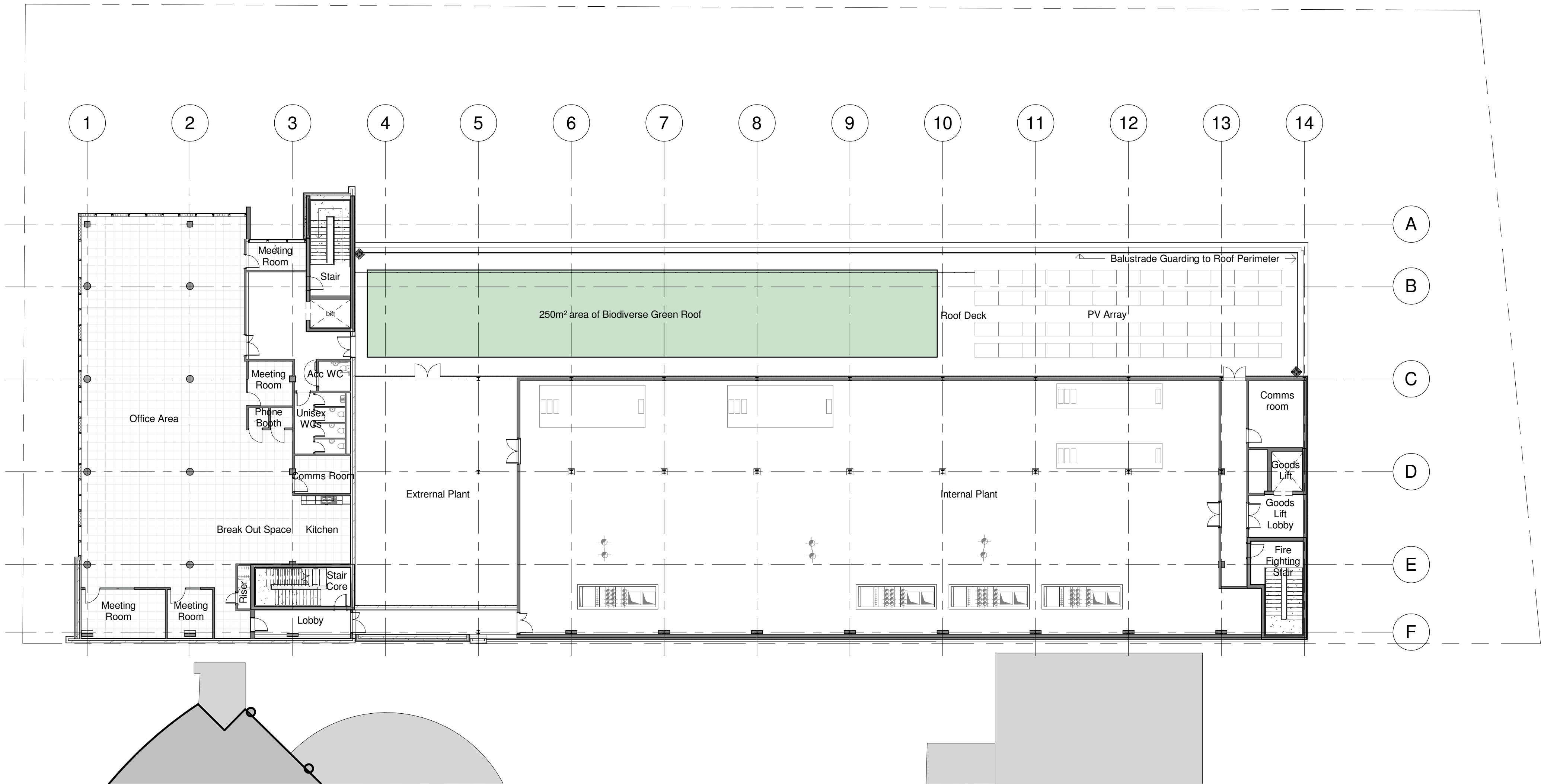
1 Proposed Second Floor Plan 1 : 200
