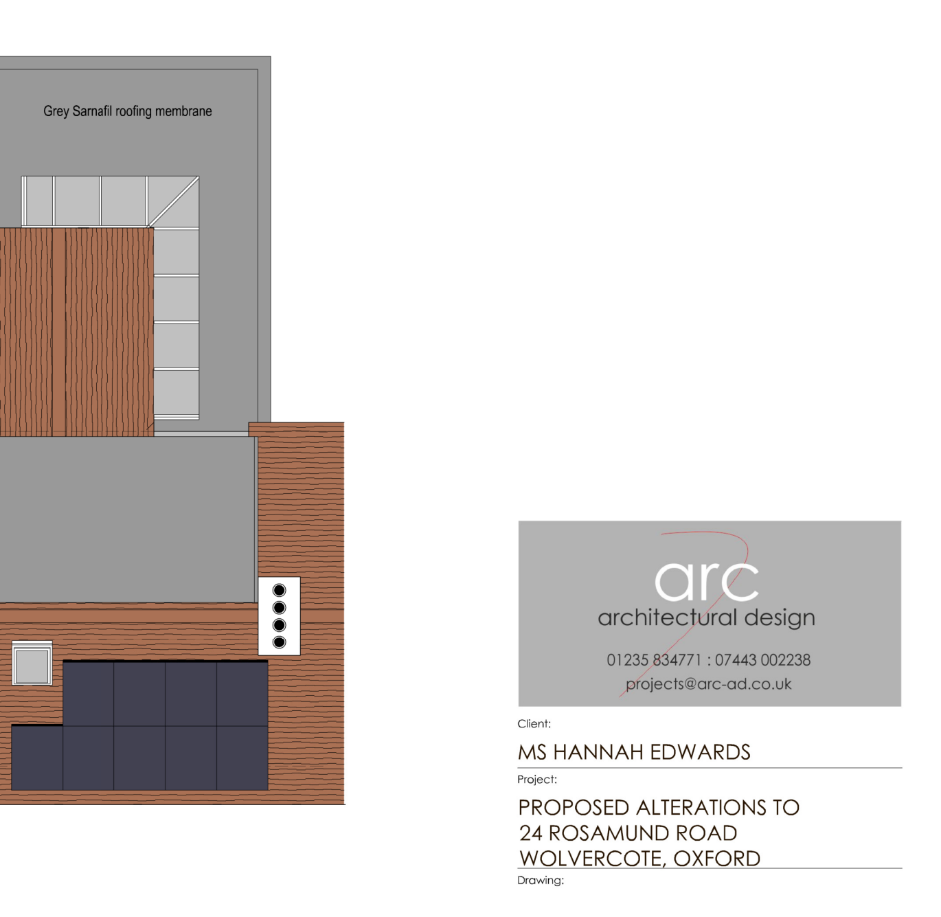
ROOF PLAN
