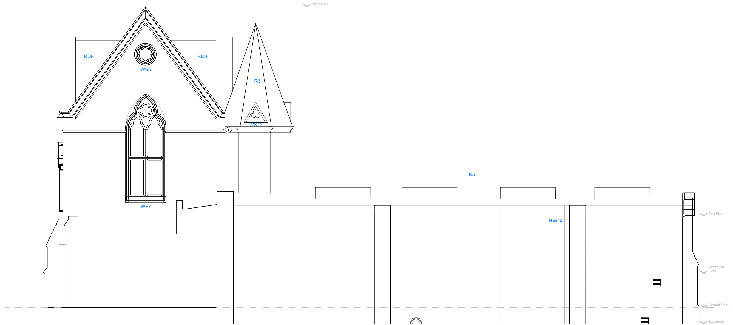
01 Existing East elevation of Main Library and Annexe 1203 1:100
