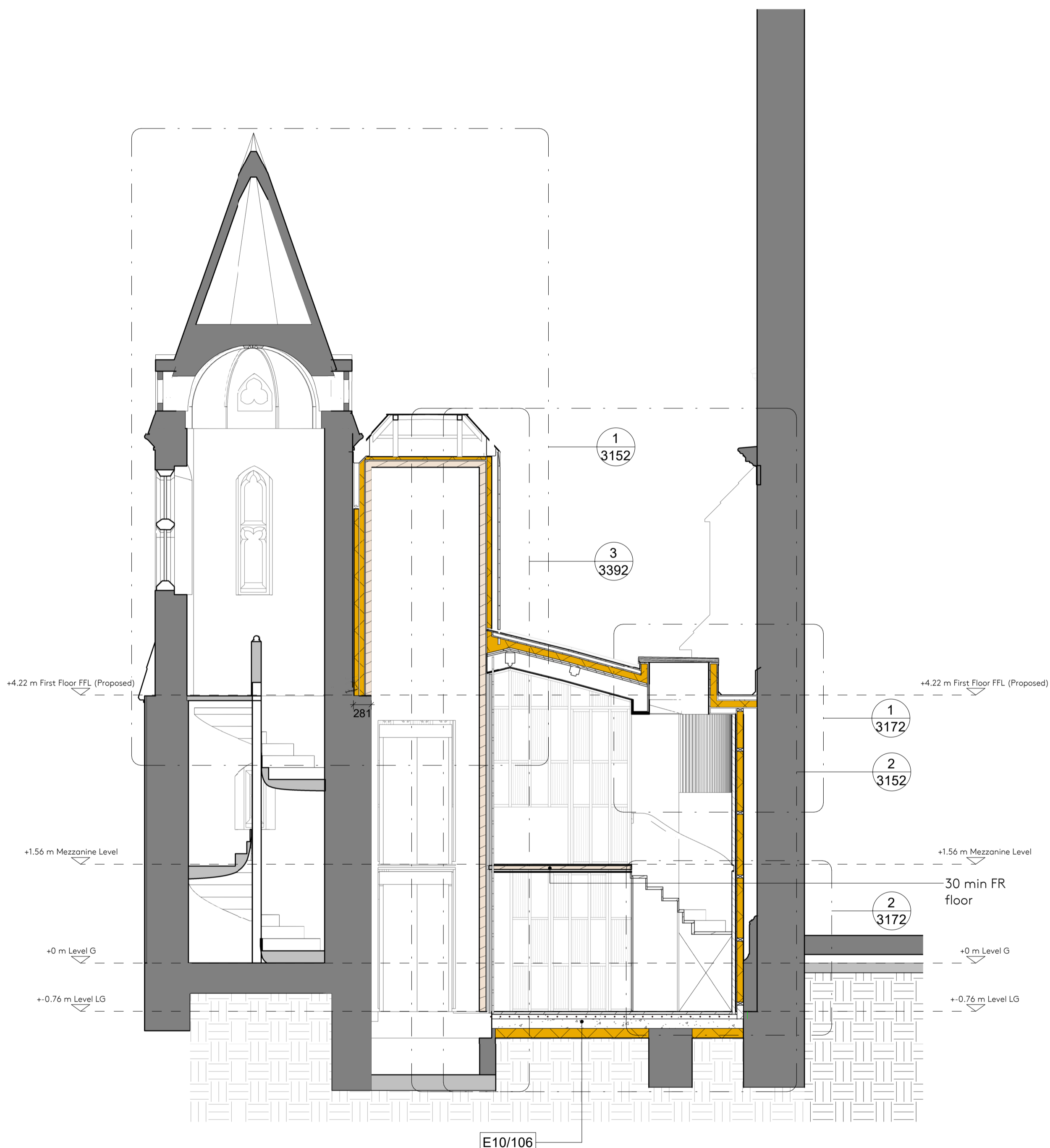
1 GA Section CC - Link CrossSec Stair 1: 50
