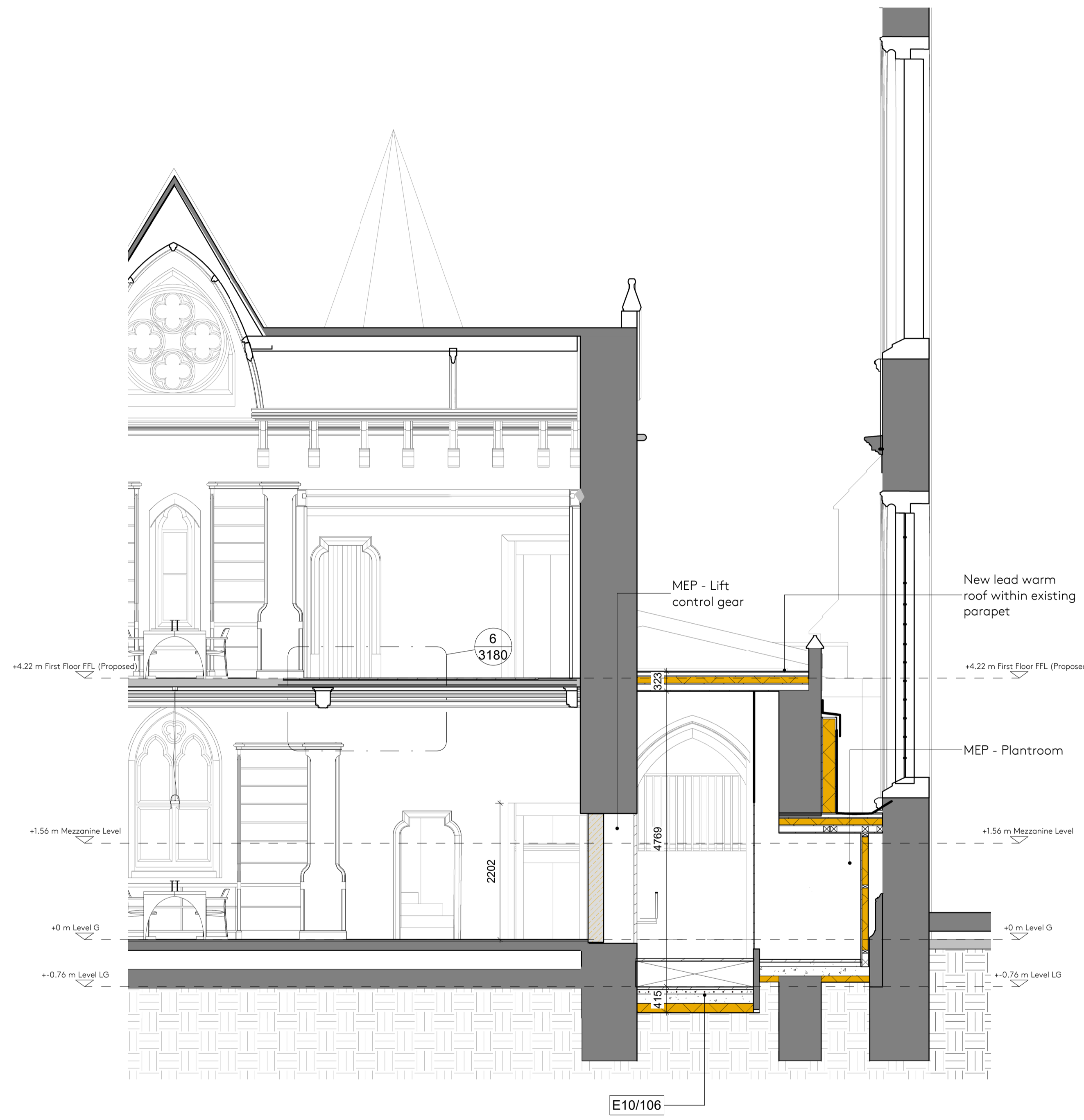
2 GA Section DD Link Cross Sec Refuge and Plantroom 1: 50
