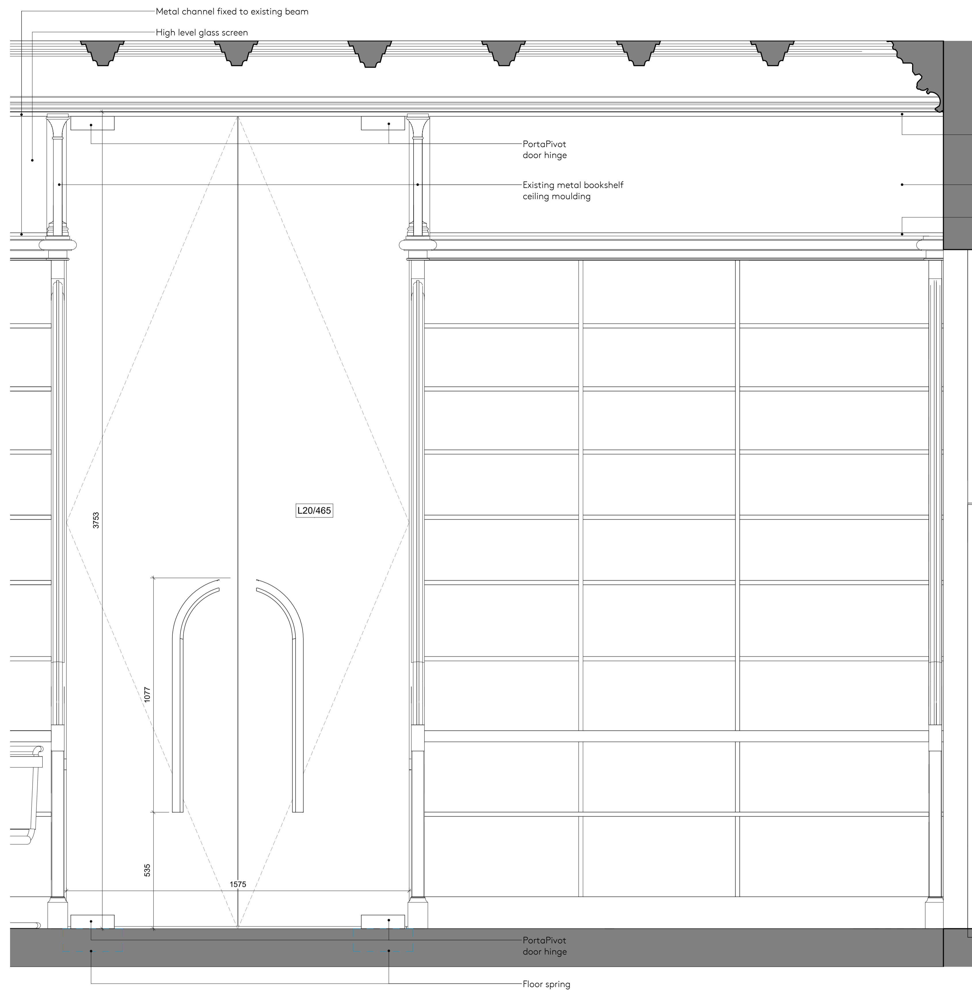
1 Main Library Internal Doors and high level screen 1 : 10
