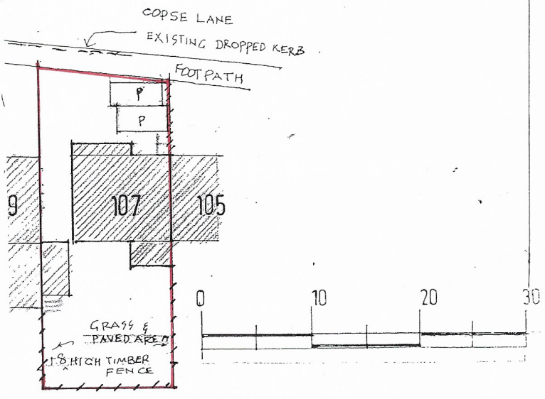
BLOCK PLAN 1:500
