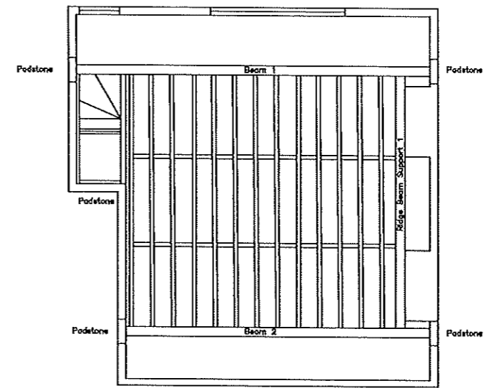
2nd Floor Floor Joists
