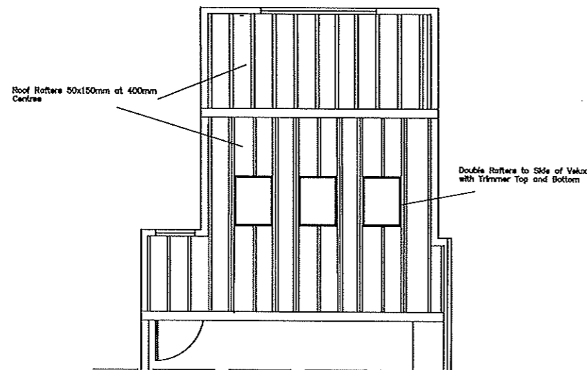
Extension Roof Rafters
