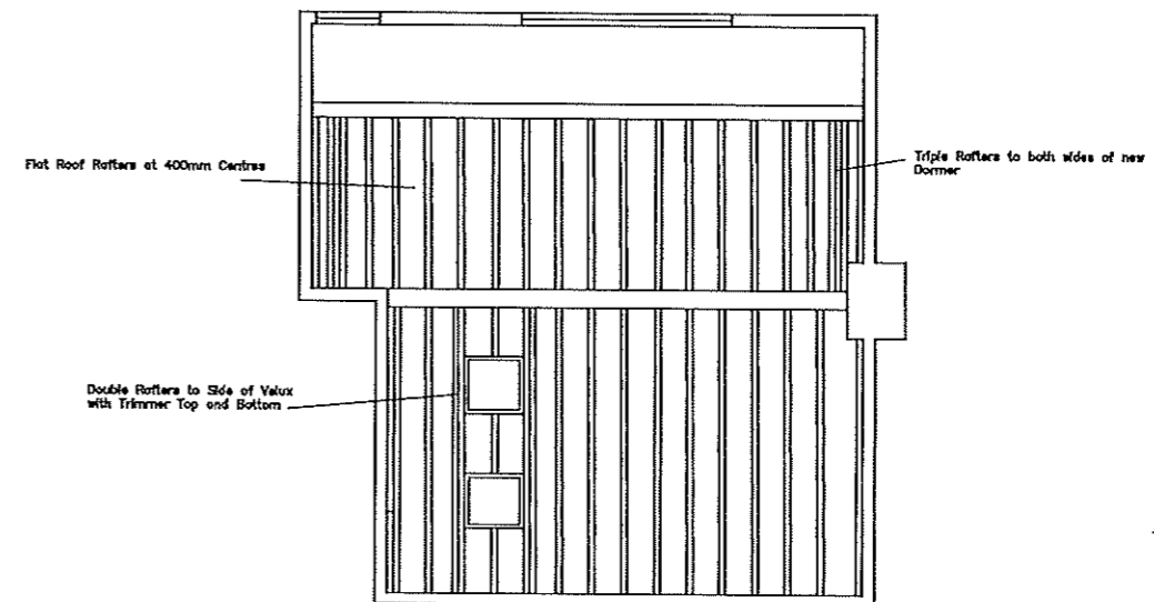
Roof Rafters
