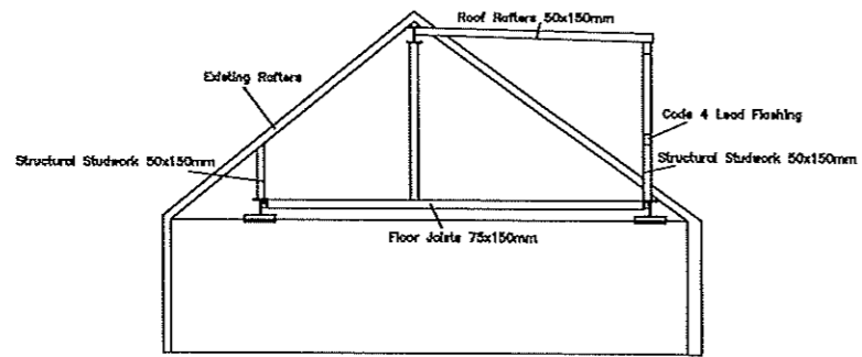
2nd Floor Side Elevation
