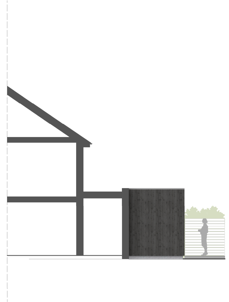
003 | proposed south / side elevation | 1:100 @ A3
