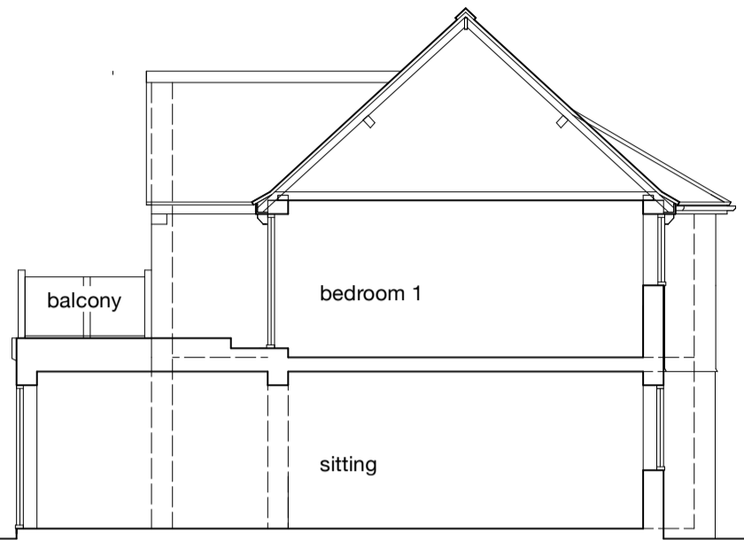
SECTION 2-2
